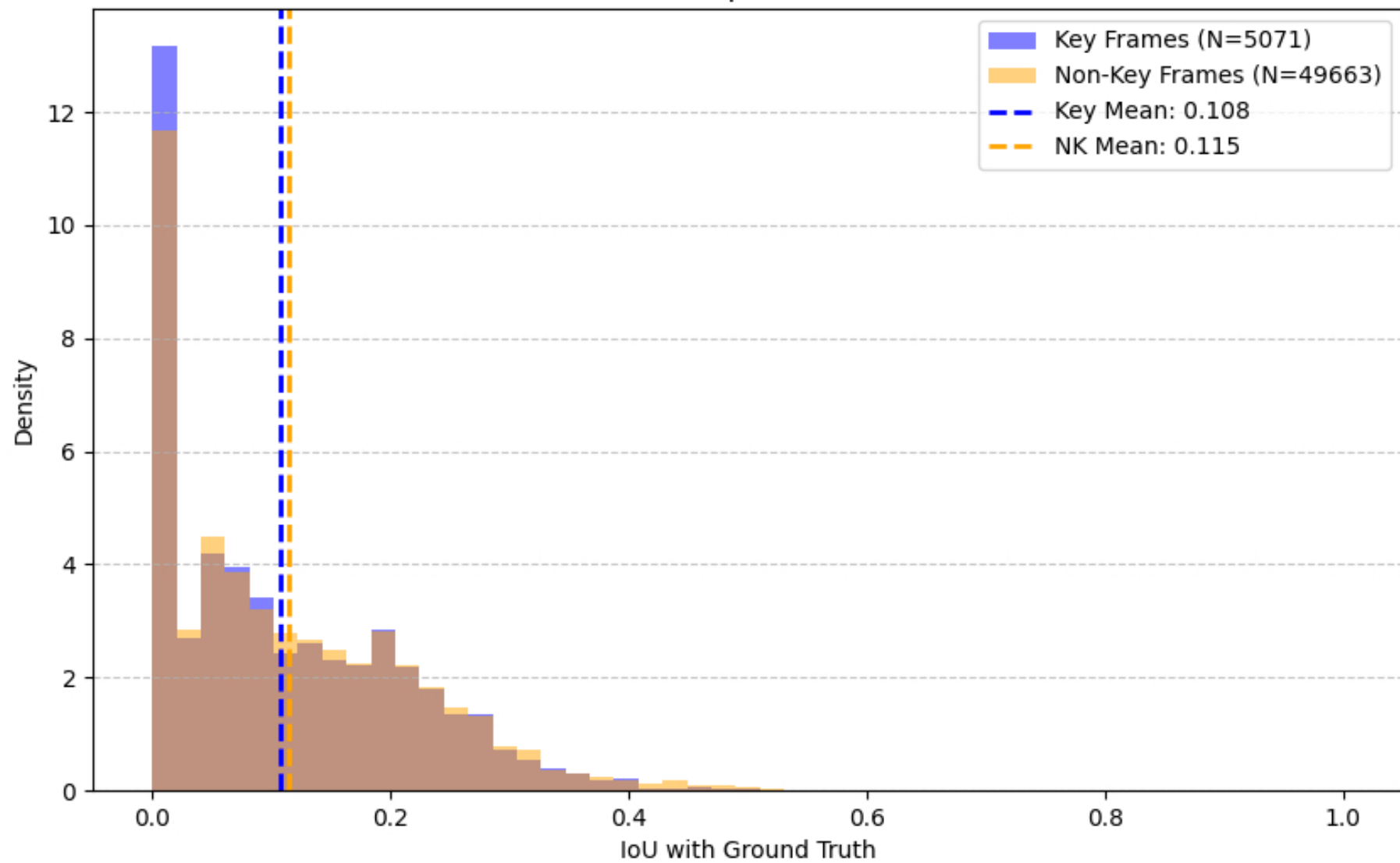
IoU Distribution Comparison (Score Thr: 0.3)
