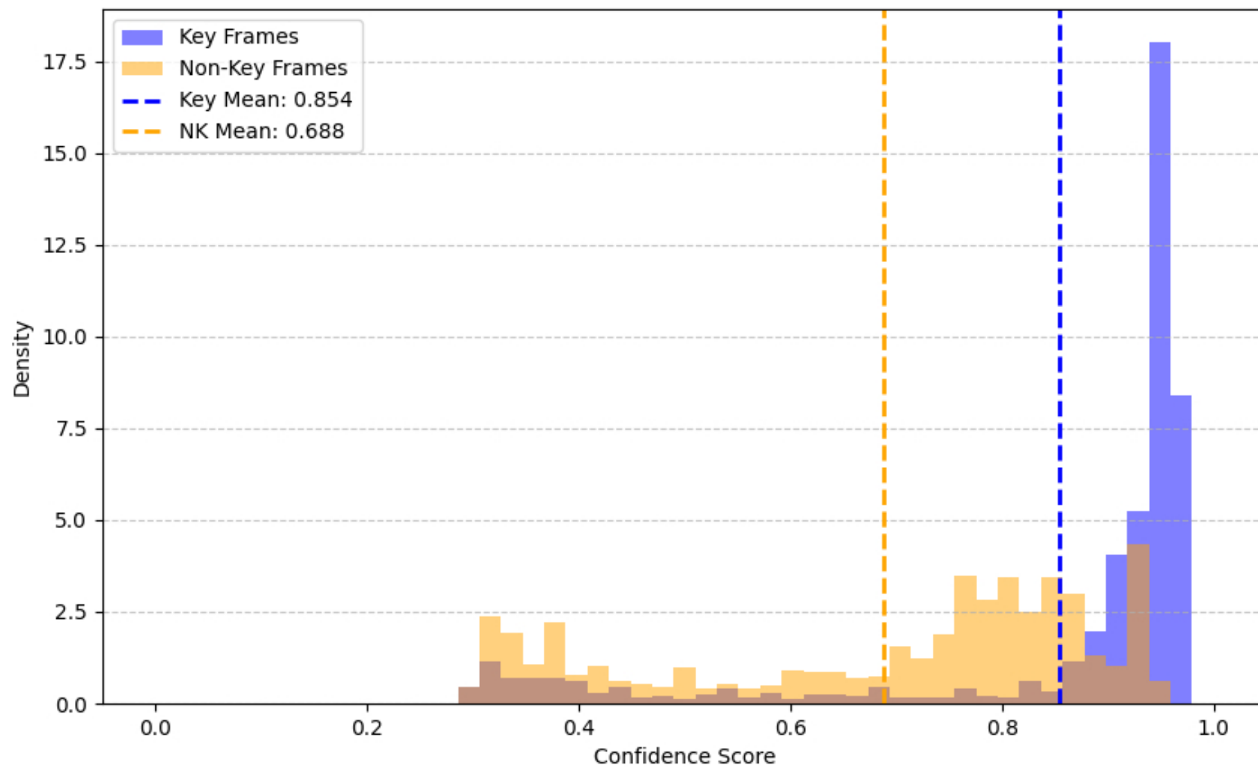
Matched Prediction Confidence Distribution
