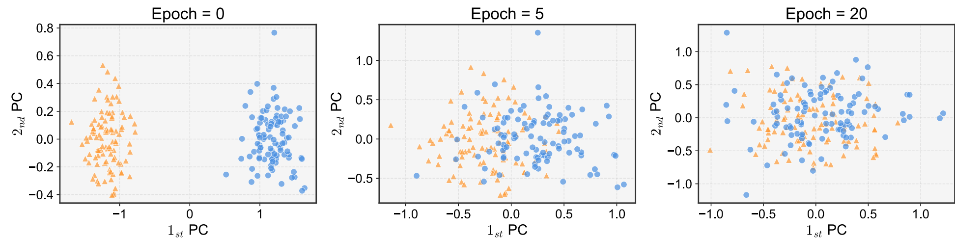
Figure: Separation between the principal components of the encoder outputs when going from power side-channel (XMEGA source device) to cache side-channel (x86 target device). The reduced differences in encoder outputs at epoch 20 indicates the presence of transferable side-channel information.
