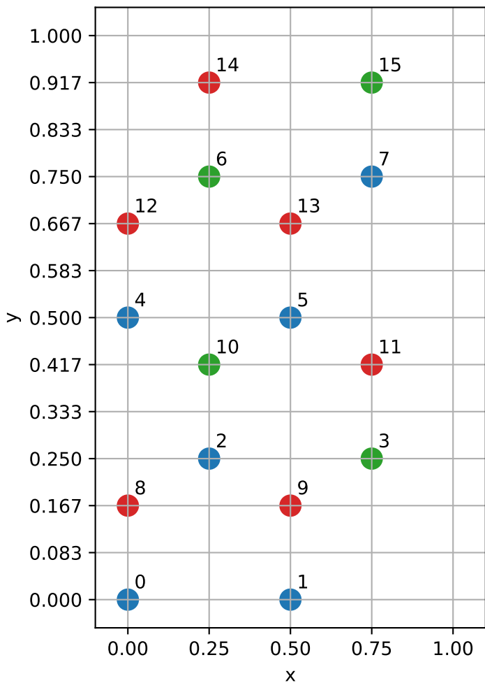
Unit cell sites (blue: z=0 , red: z=0.5 )
