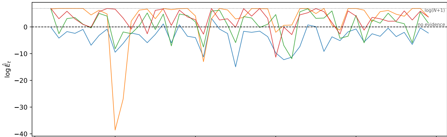
Synthetic validation, corrected estimator ( N = 1000 , identity adjoined)
