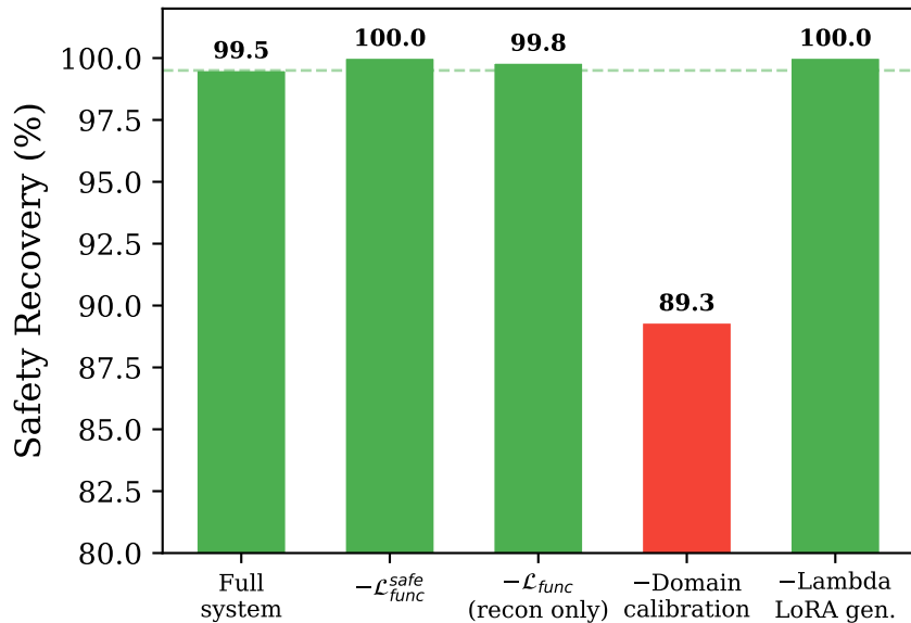
Safety Recovery ↑
