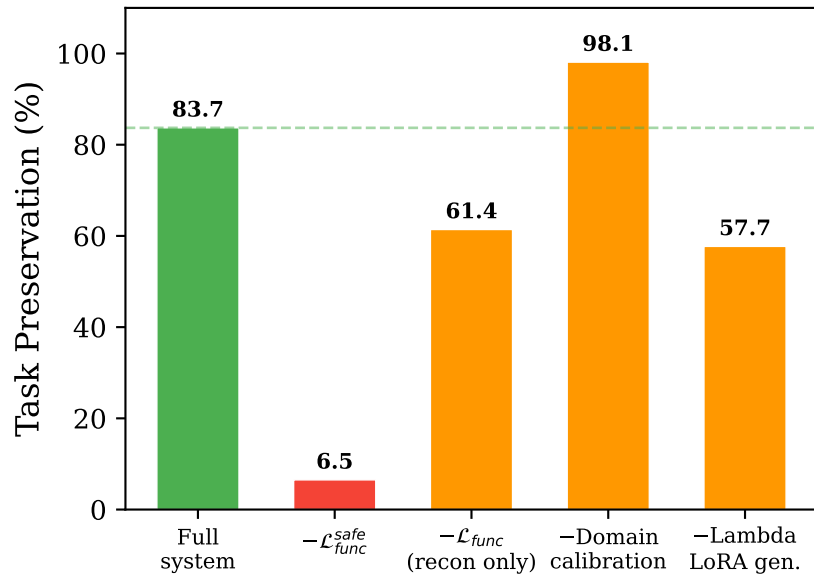
Task Preservation ↑
