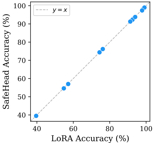
Qwen2-7B
