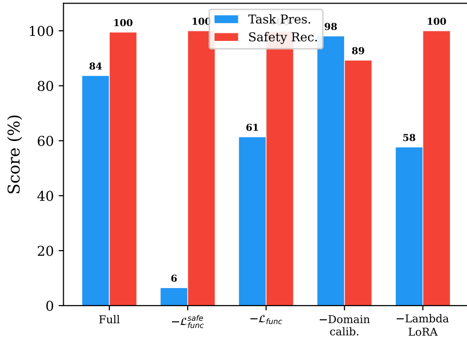
(a) Component Ablation
