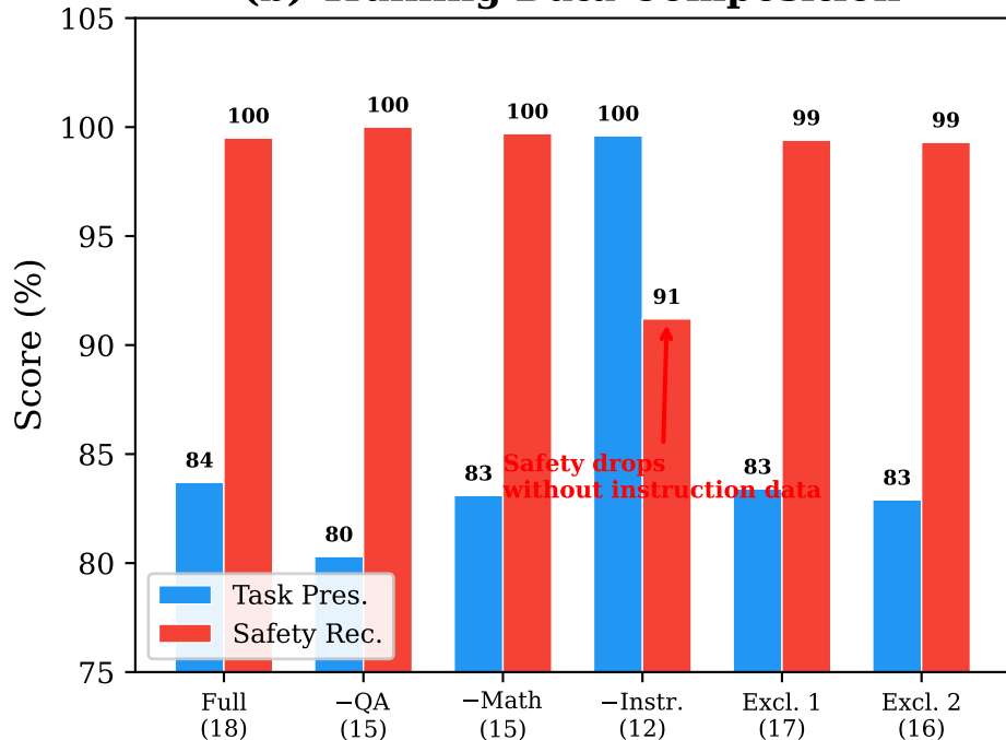
(b) Training Data Composition
