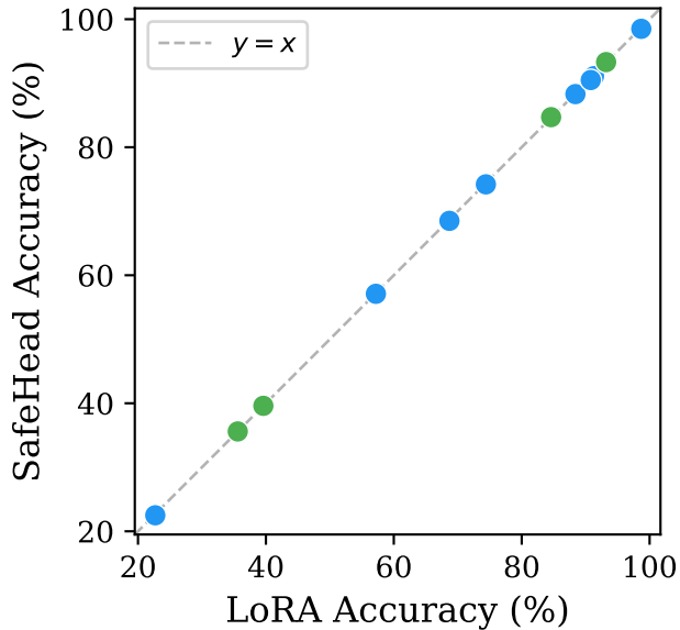
Qwen2-7B
