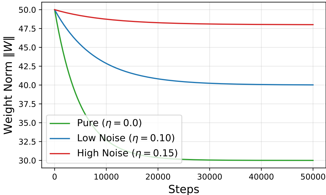
Weight Norm Evolution vs Noise
