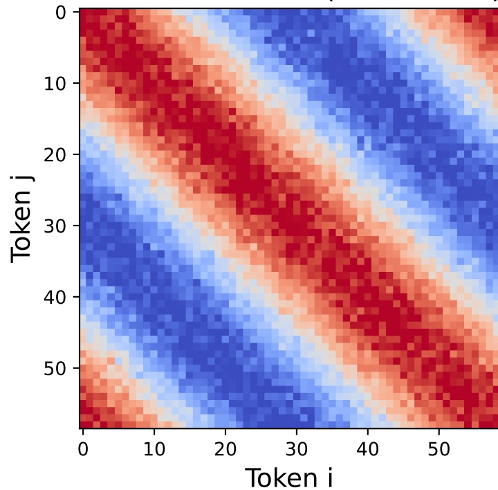
Pure Model RSM (Structured)
