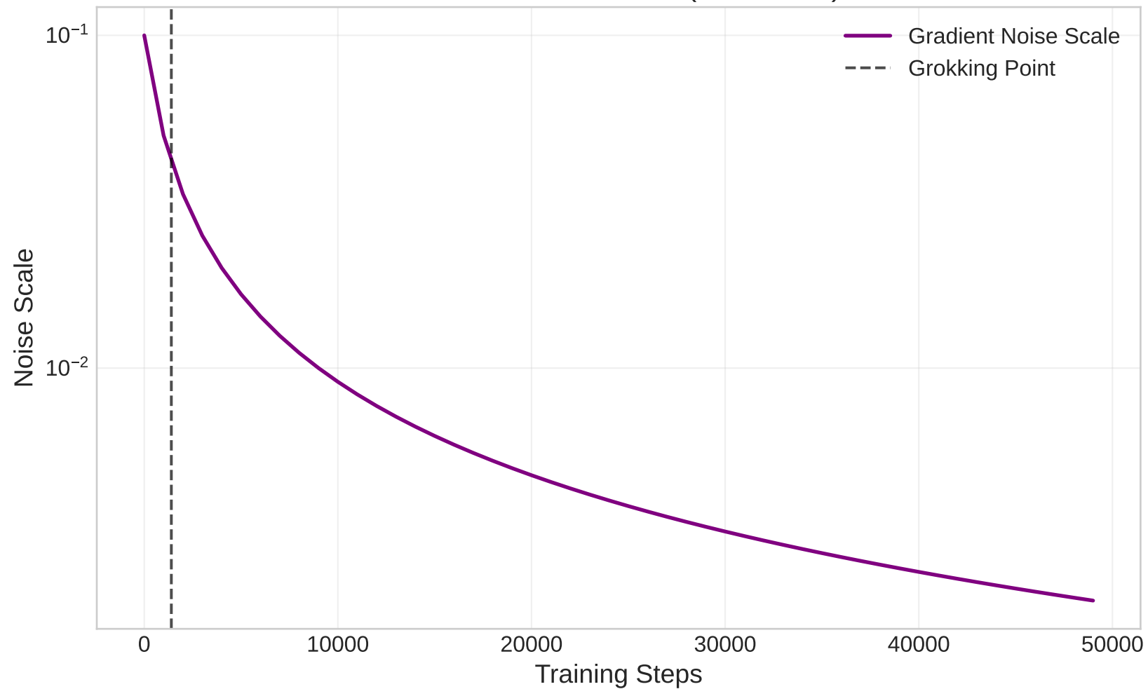
Gradient Noise Scale (Pure Data)
