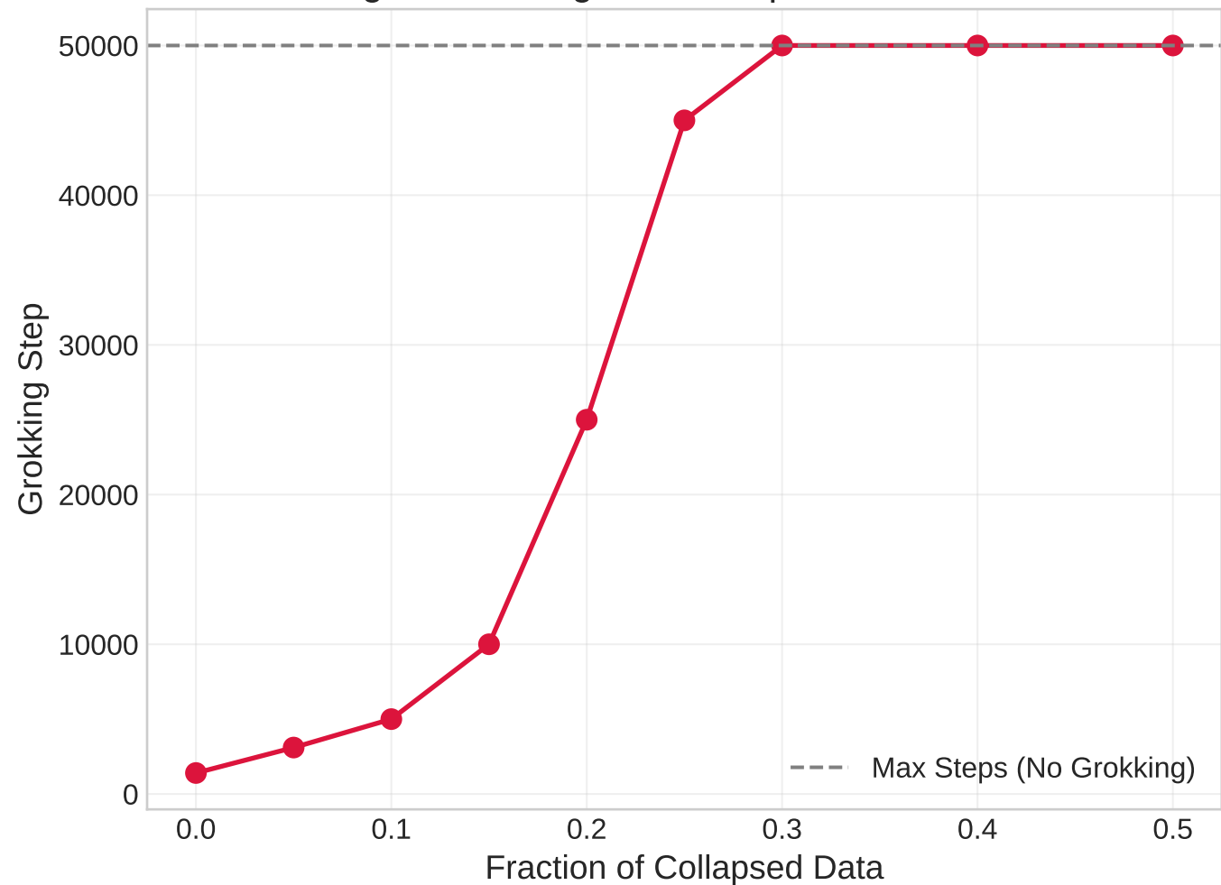
Grokking Phase Diagram: Collapse vs Generalization
