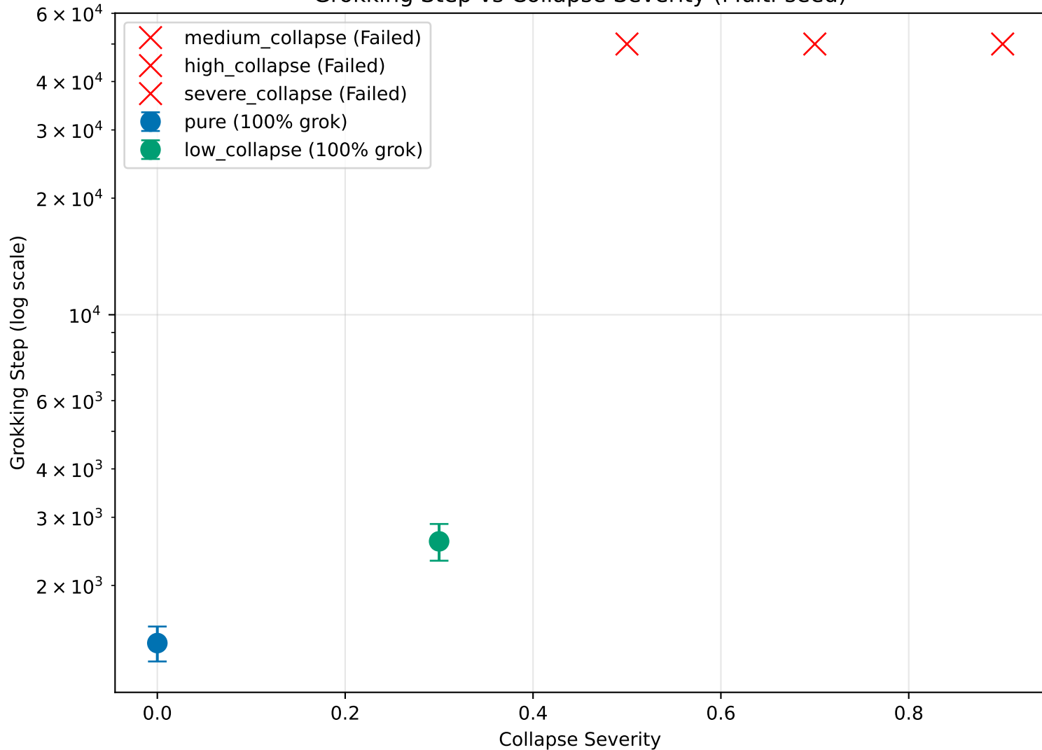
Grokking Step vs Collapse Severity (Multi-seed)
