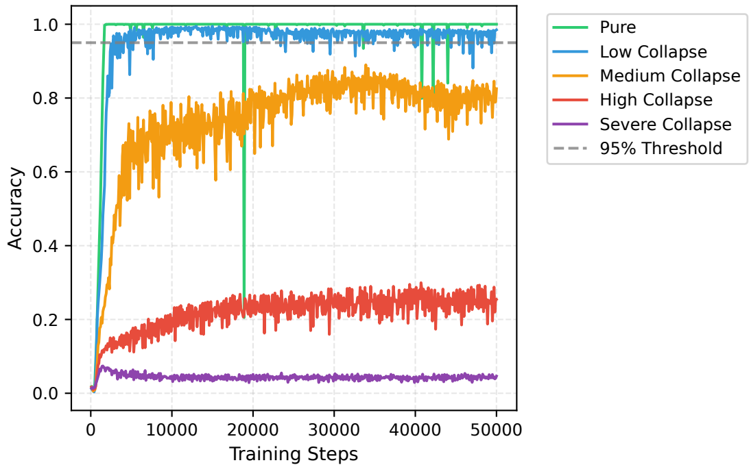
Test Accuracy (Grokking)
