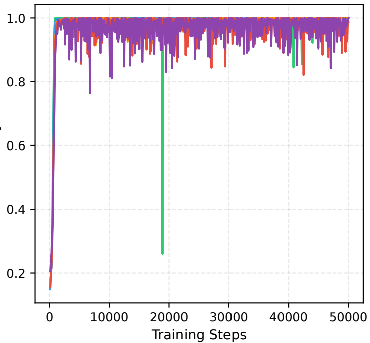
Train Accuracy
