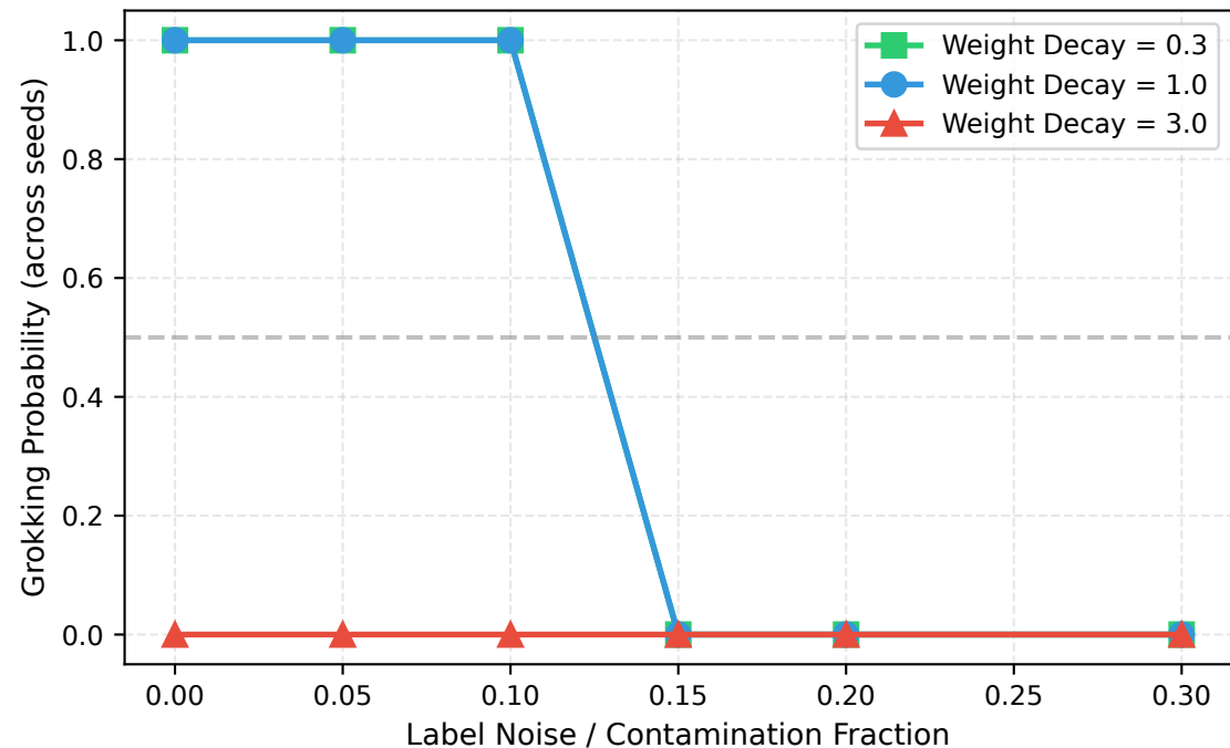
The Grokking Cliff
