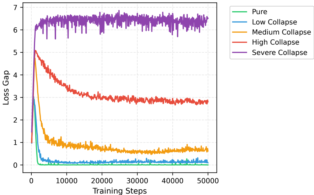
Generalization Gap (Test Loss - Train Loss)
