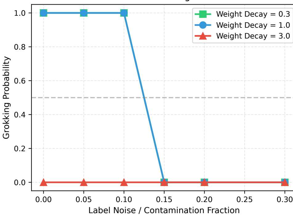
D. The Grokking Cliff
