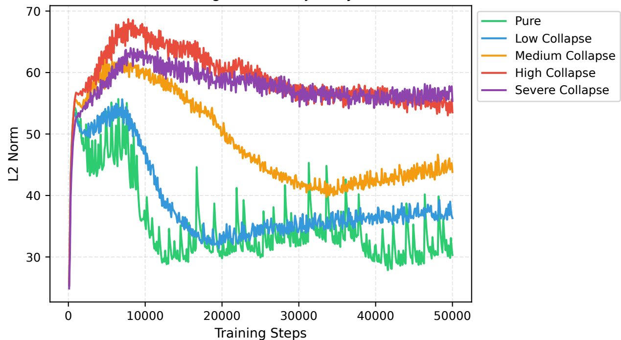
D. The Grokking Cliff
