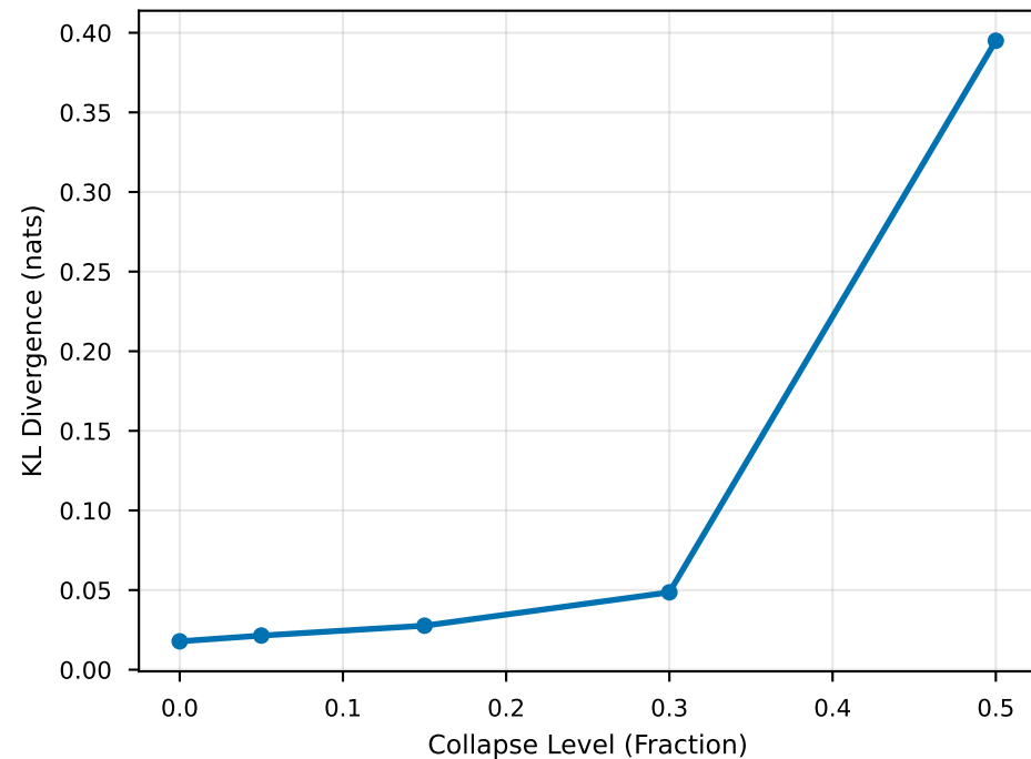
Distribution Shift vs Collapse
