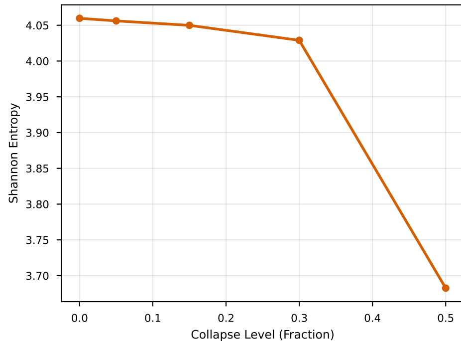
Target Diversity vs Collapse
