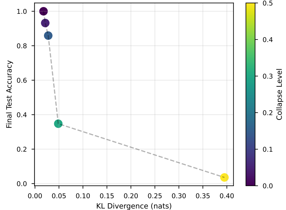
Grokking Success vs Data Quality
