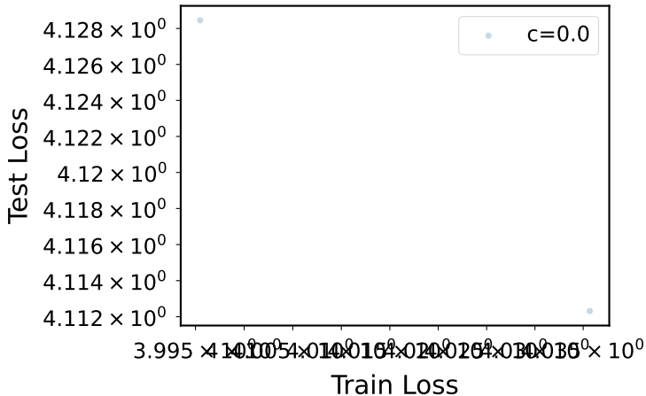
Loss Trajectories
