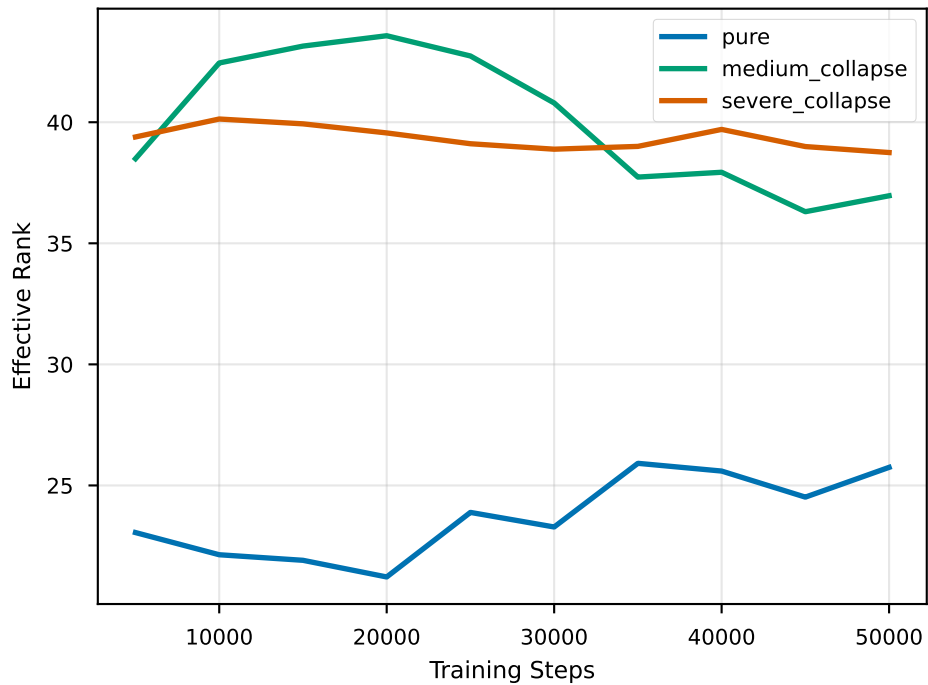
Token Embedding Rank Evolution
