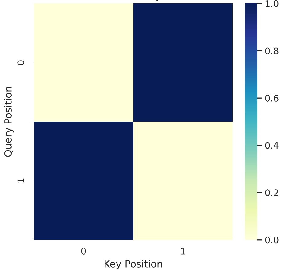
Collapsed - Early
