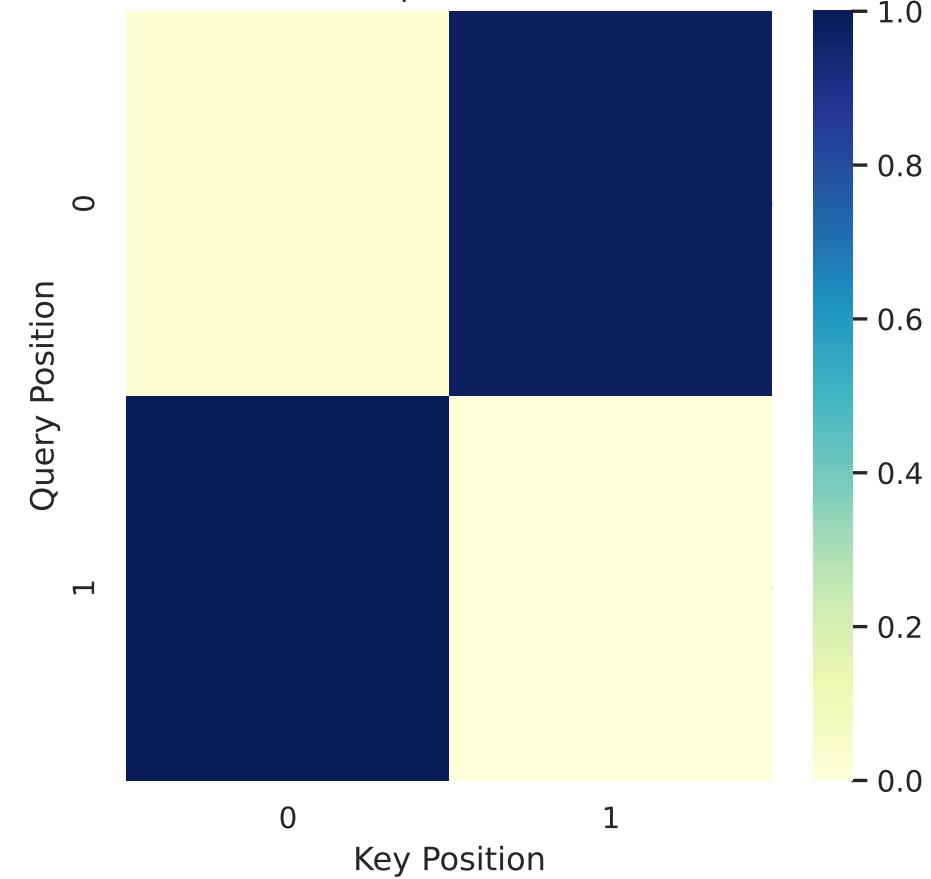
Collapsed - Late
