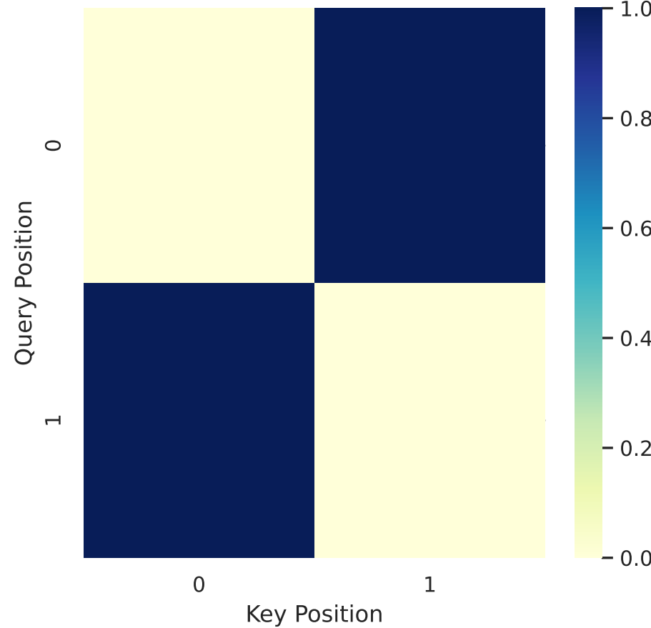
Collapsed - Mid
