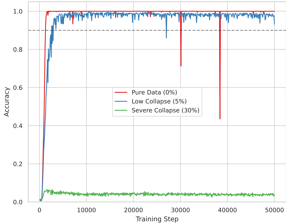
Test Accuracy (Grokking)
