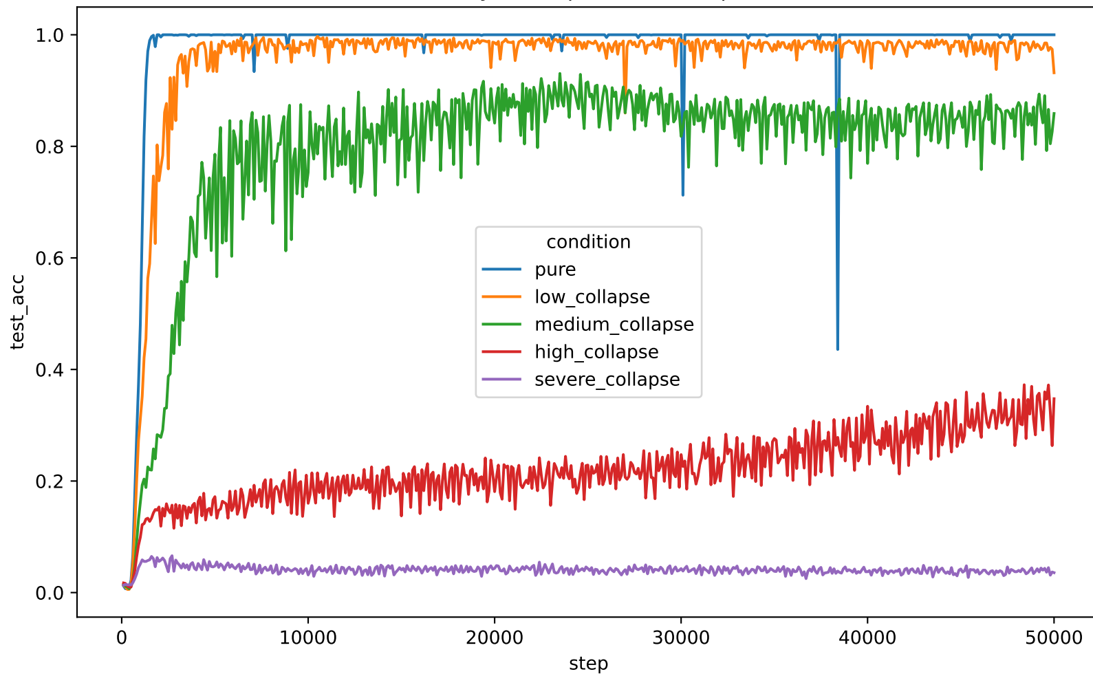
Test Accuracy vs Step across Collapse Levels
