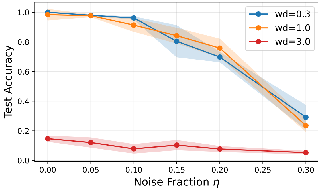
Test Accuracy vs Noise (Grokking Cliff)
