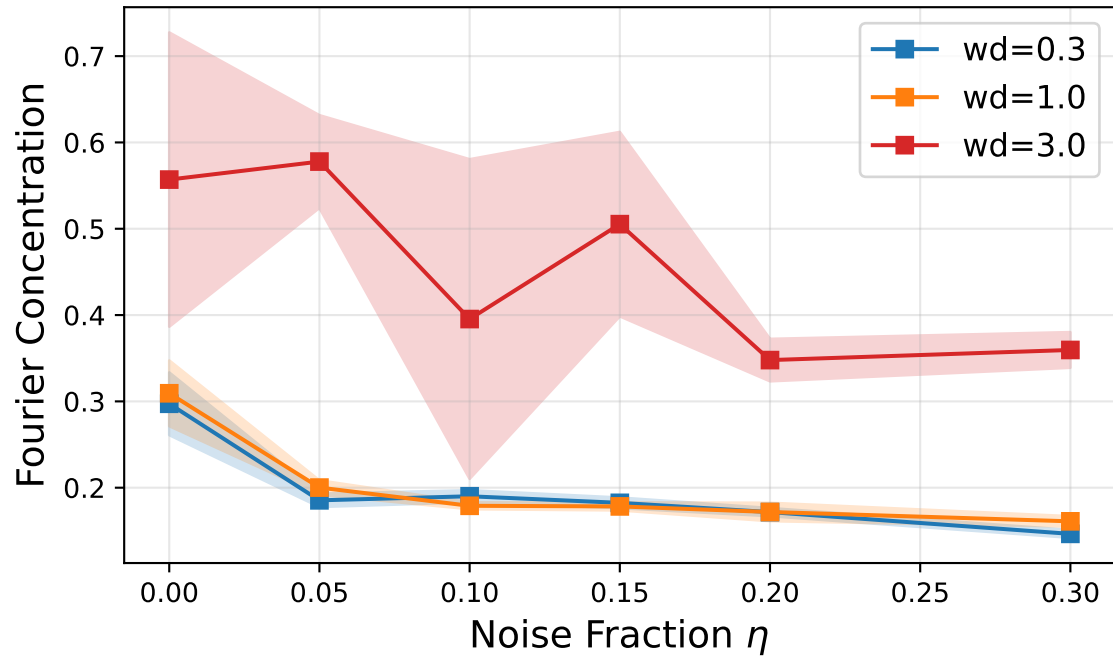
Fourier Concentration vs Noise
