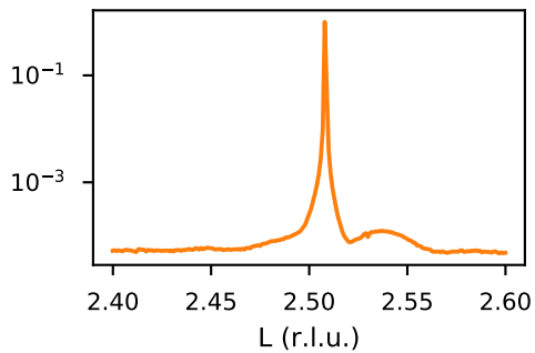
(1/2 1/2 5/2)
