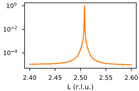
(5/2 1/2 1/2)
