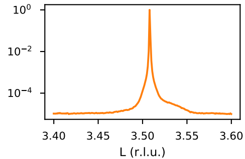
(1/2 1/2 7/2)
