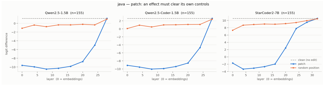
Figure 21: Boolean patch layer profiles for Java across all three models and available controls.
