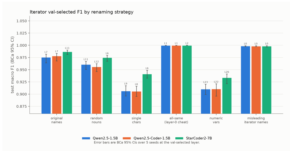
Figure 59: Iterator val-selected F1 by renaming strategy, with BCa 95% intervals.
