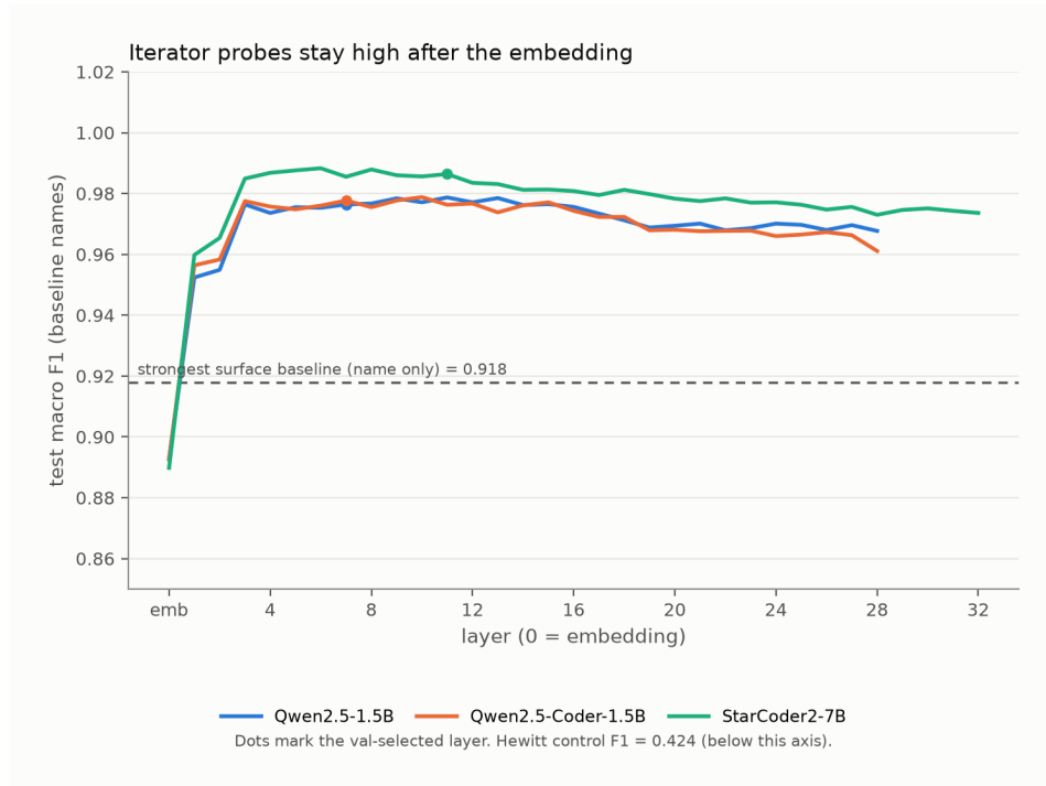
Figure 53: Iterator probe macro-F1 across layers on original names, with the name-only surface baseline marked.
