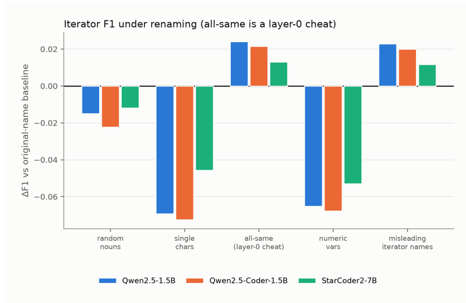
Figure 54: Iterator perturbation deltas relative to baseline.
