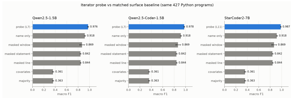
Figure 57: Iterator probe versus matched model-free surface baselines on the same 427 Python programs.
