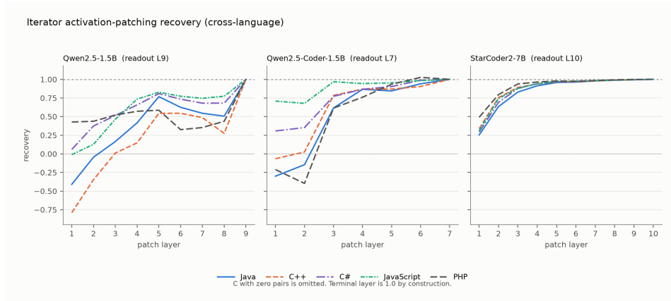
Figure 62: Exploratory iterator activation-patching recovery under cross-language transfer. C-language rows with zero pairs are omitted.
