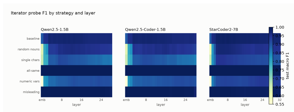
Figure 60: Iterator probe F1 by strategy and layer.
