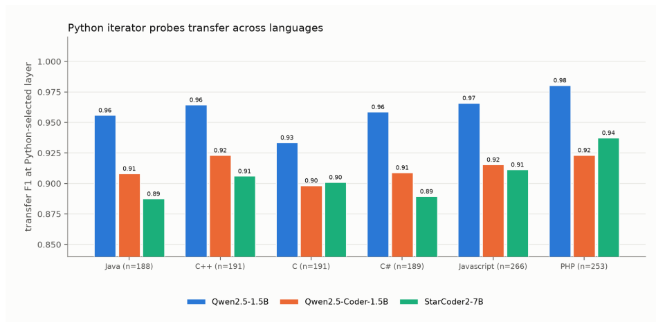
Figure 56: Available iterator cross-language transfer results.
