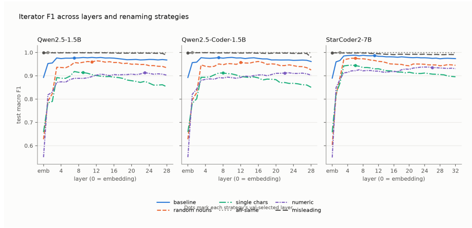
Figure 58: Iterator probe macro-F1 across layers and renaming strategies.
