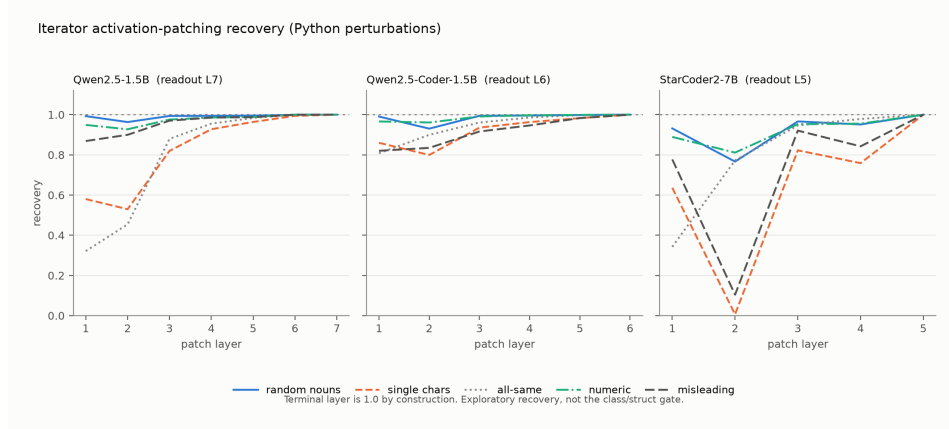
Figure 61: Exploratory iterator activation-patching recovery under Python name perturbations. The terminal layer is one by construction.
