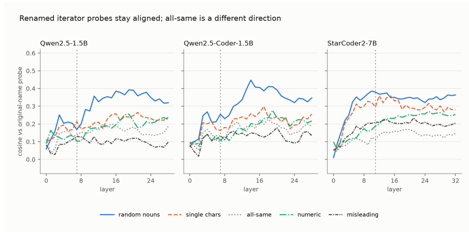
Figure 55: Iterator cosine similarity to the baseline direction.
