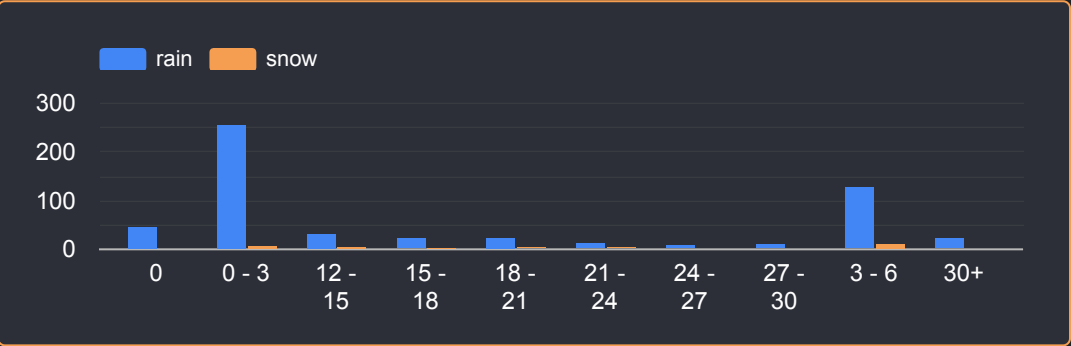
Precipitation on Rainy and Snowy Days
