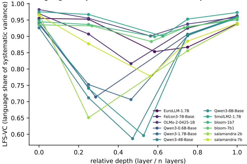
The language component across Transformer depth (14 models)
