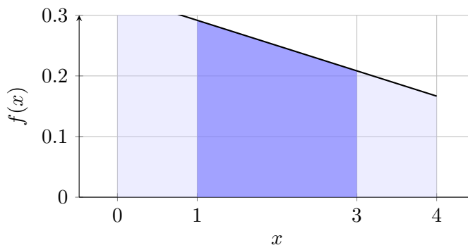
Band graph: P(1 \leq X \leq 3)
