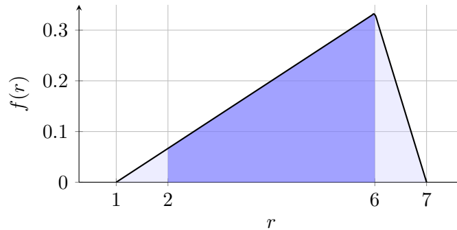
Band graph: P(2 \leq R \leq 6)
