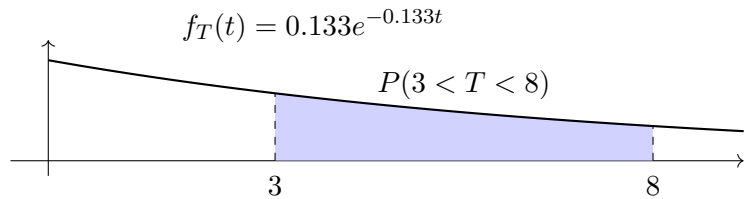
Probability region
