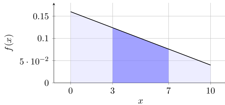
Band graph: P(3 \leq X \leq 7)
