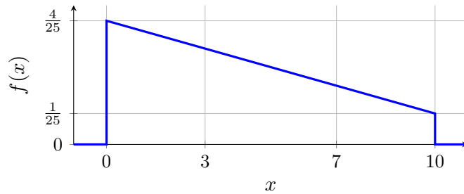
Completed density graph
