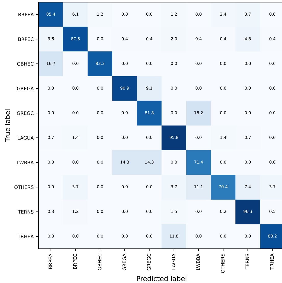
Validation
