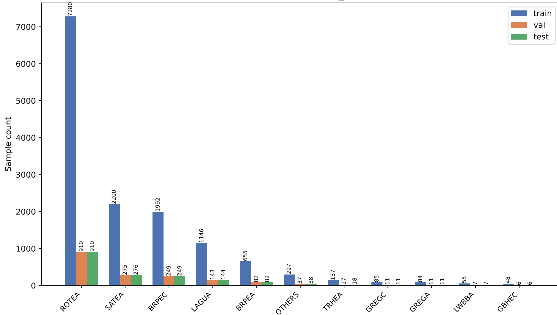
Split distribution — exp1_11class
