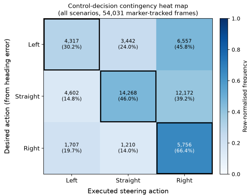
Figure 4.15: Control-decision contingency heat map (pooled over all four scenarios, 54,031 marker-tracked frames). Rows are the desired corrective action implied by the instantaneous heading error ( \pm 5^\circ dead-band) and columns are the executed steering action; cells are shaded by row-normalized frequency and annotated with frame counts and row percentages. The diagonal cells (instantaneous agreement) are outlined. The substantial off-diagonal mass in the Straight row reflects anticipatory, phase-lagged steering rather than tracking failure.
