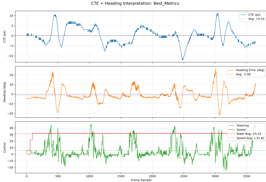
Figure 4.9: Physical deployment of the Egocentric Dynamic Crop Model resulted in successful navigation through the entire track, with stable CTE and Heading Error profiles.
