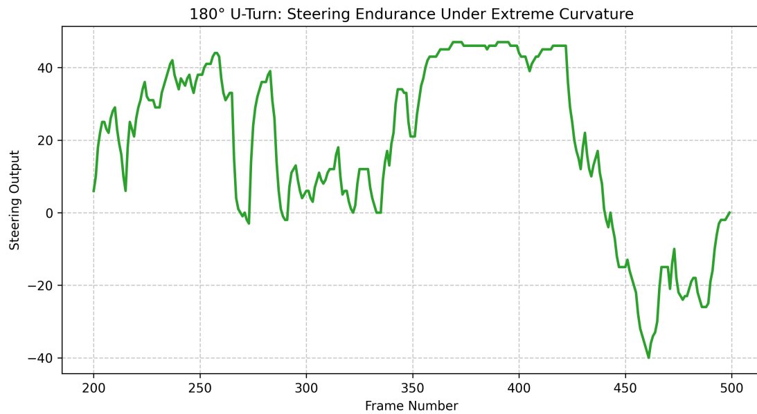
Figure 4.12: 180-degree U-turn telemetry illustrating sustained steering actuation under extreme curvature.
