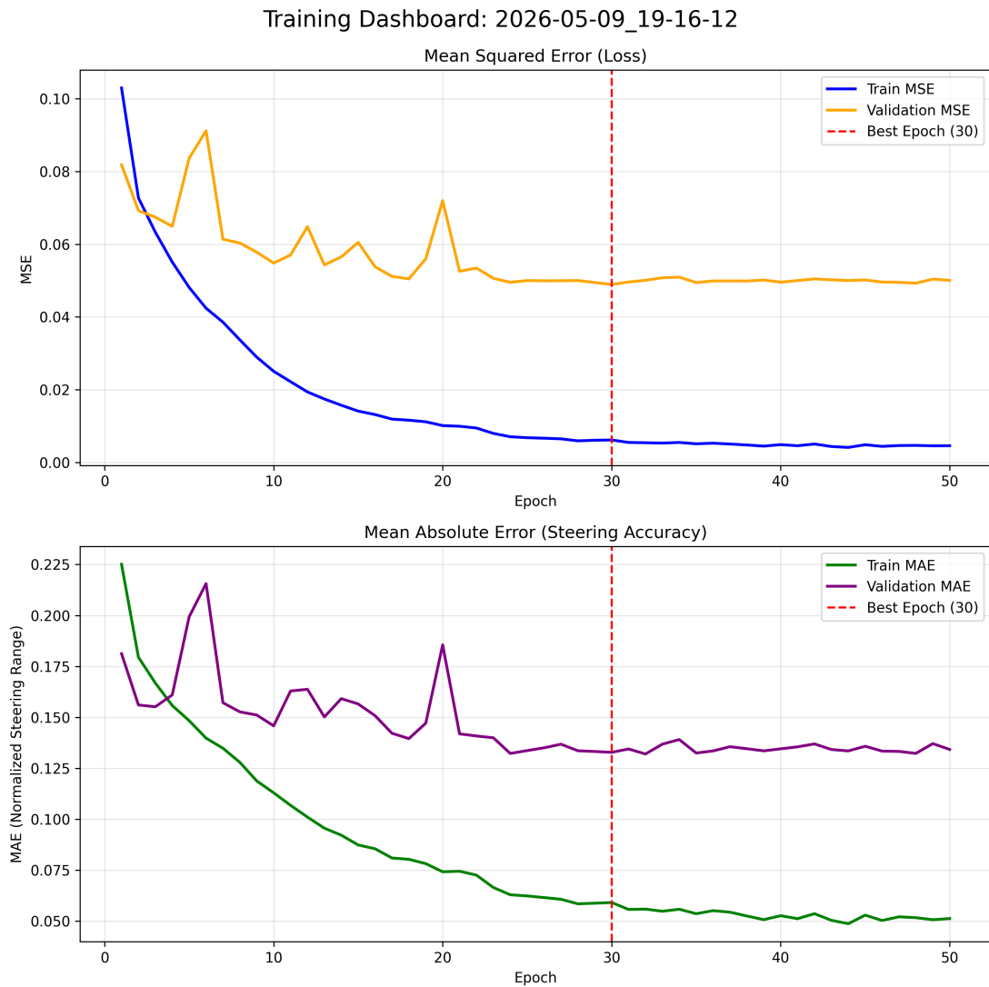
Figure 4.2: The near-perfect convergence of MSE and MAE suggested successful learning, though this was later identified as spatial memorization.
