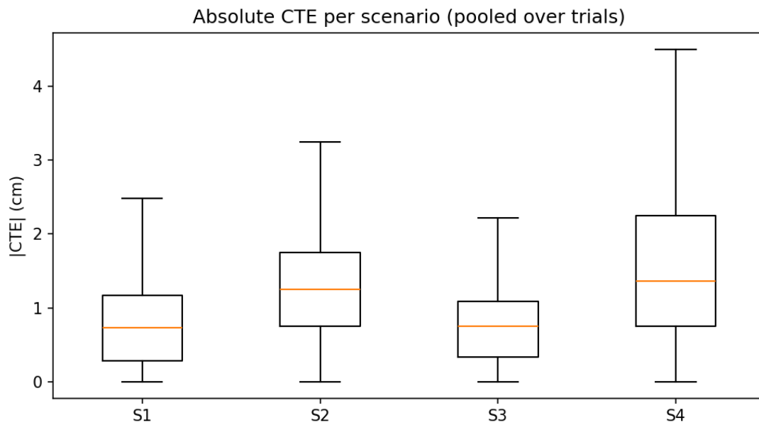
Figure 4.14: Distribution of absolute Cross-Track Error (cm) per scenario, pooled over N = 10 trials each, including the held-out track. Error scales with curvature severity and rises on the unseen topology while remaining bounded.
