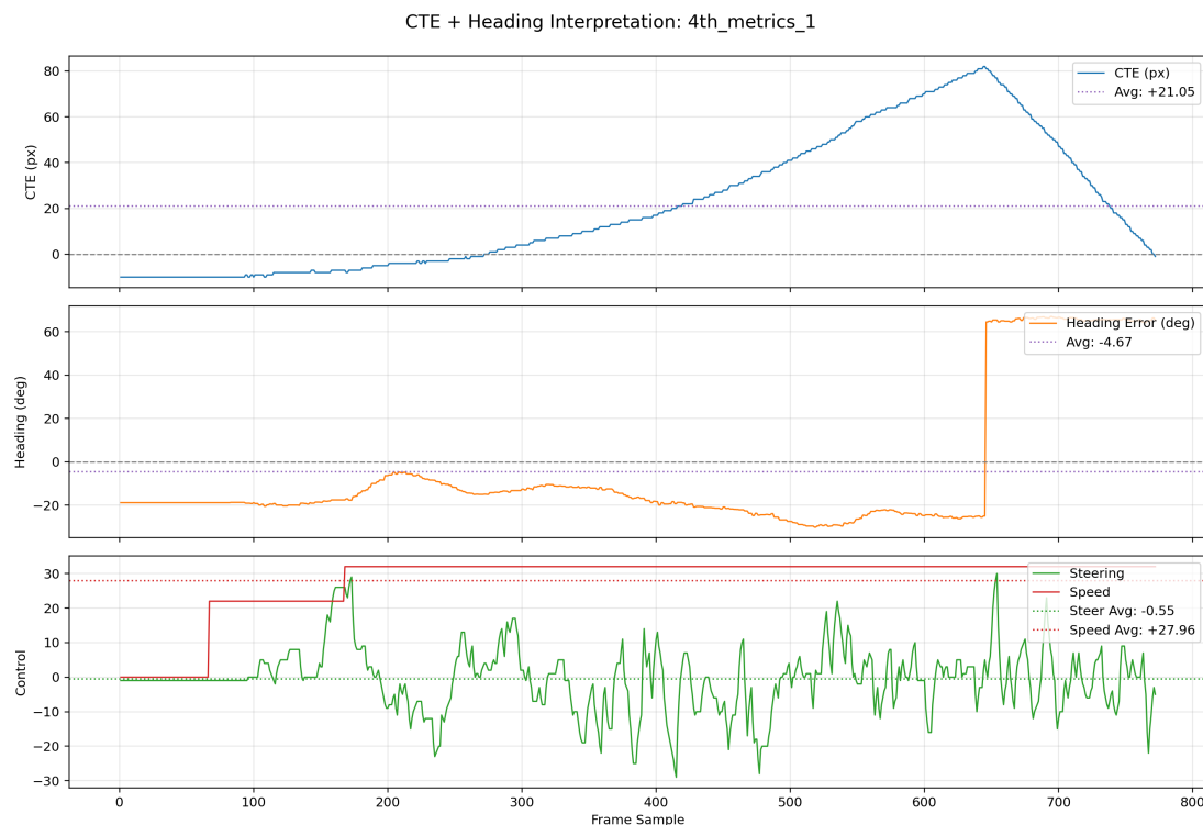
Figure 4.6: Limited real-world trial for Baseline B. CTE drifted upward with a late-stage heading discontinuity, while steering oscillations persisted under increasing speed.
