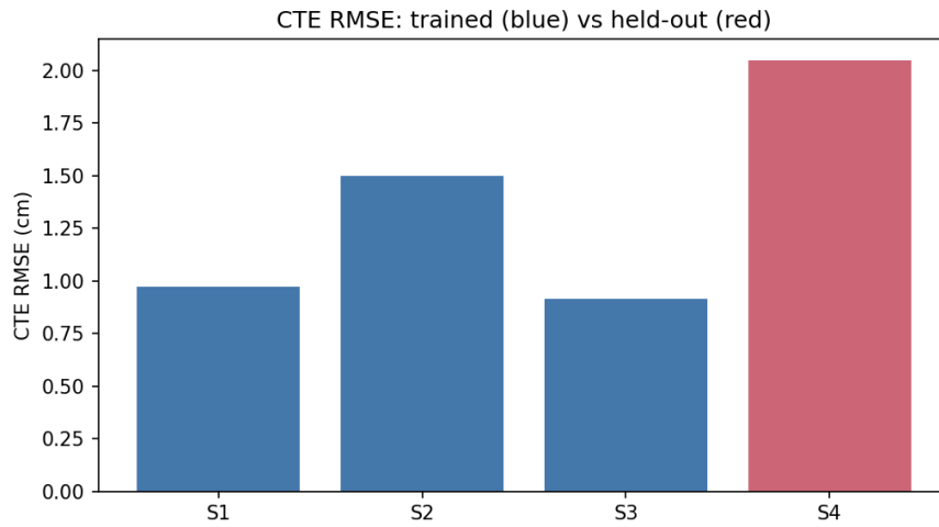
Figure 4.13: Generalization: CTE RMSE on the trained tracks (pooled, N = 30 ) versus the held-out track ( N = 10 ). Error grows 1.70\times on the unseen topology while success remains at 100%.
