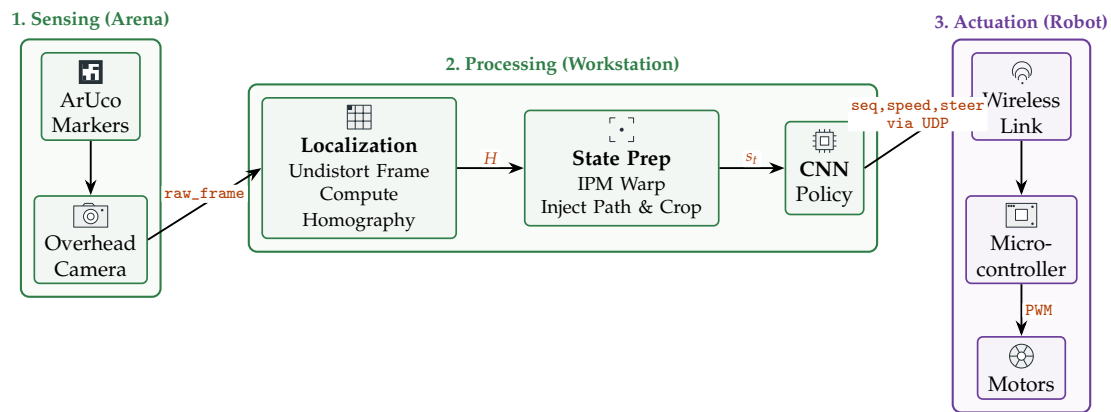
Figure 3.10: End-to-end system processing pipeline. Boxes denote processing stages grouped into the sensing, processing, and actuation zones; labels on the arrows name the data structure passed between stages (see Table 3.1): the raw frame is localized into a homography H , prepared into the normalized state s_t , mapped by the CNN to a control vector, and transmitted over UDP to the robot.
