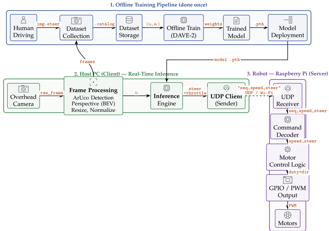
Figure 3.9: Client-server hardware architecture of the autonomous navigation system. The Host PC (client, green) performs offline training (blue, done once) and real-time inference, transmitting the serialized control command to the onboard Raspberry Pi (server, purple) over UDP. Arrow labels name the data structure passed at each step (cf. Table 3.1).
