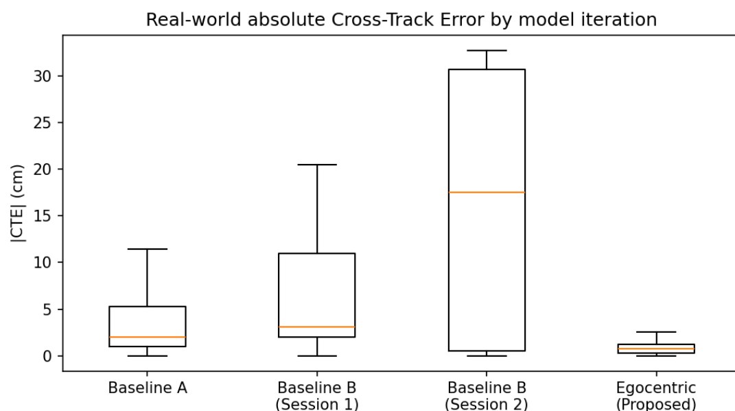
Figure 4.10: Real-World Trajectory Deviations: absolute Cross-Track Error (cm) box plot across model iterations.
