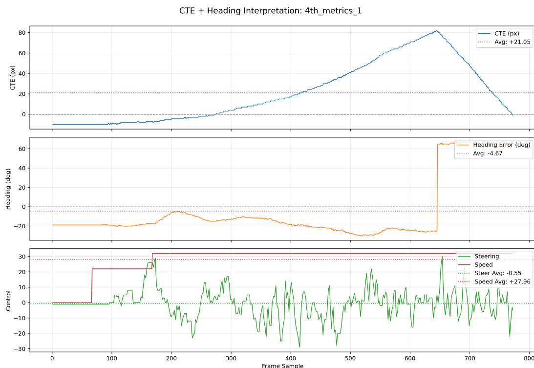
Figure 4.6: Limited real-world trial for Baseline B. CTE drifted upward with a late-stage heading discontinuity, while steering oscillations persisted under increasing speed.
