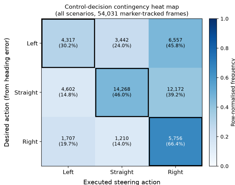
Figure 4.12: Control-decision contingency heat map (pooled over all four scenarios, 54,031 marker-tracked frames). Rows are the desired corrective action implied by the instantaneous heading error ( \pm 5^\circ dead-band) and columns are the executed steering action; cells are shaded by row-normalized frequency and annotated with frame counts and row percentages. The diagonal cells (instantaneous agreement) are outlined. The substantial off-diagonal mass in the Straight row reflects anticipatory, phase-lagged steering rather than tracking failure.
