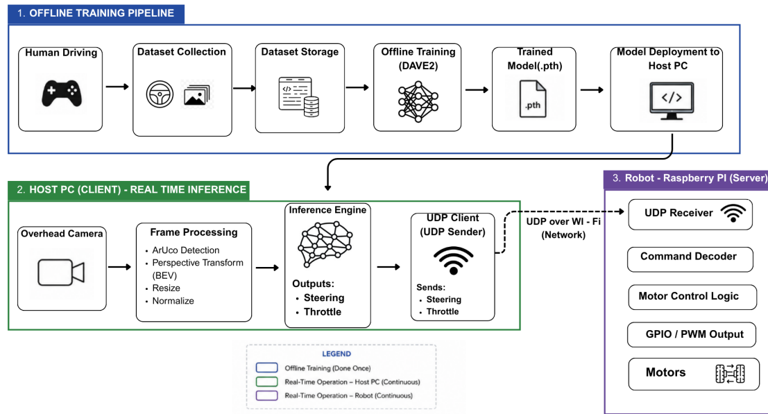
Figure 3.9: Client-server hardware architecture of the autonomous navigation system. The Host PC (client) handles all perception, offline training, and real-time inference, transmitting control commands to the onboard Raspberry Pi (server) over UDP.
