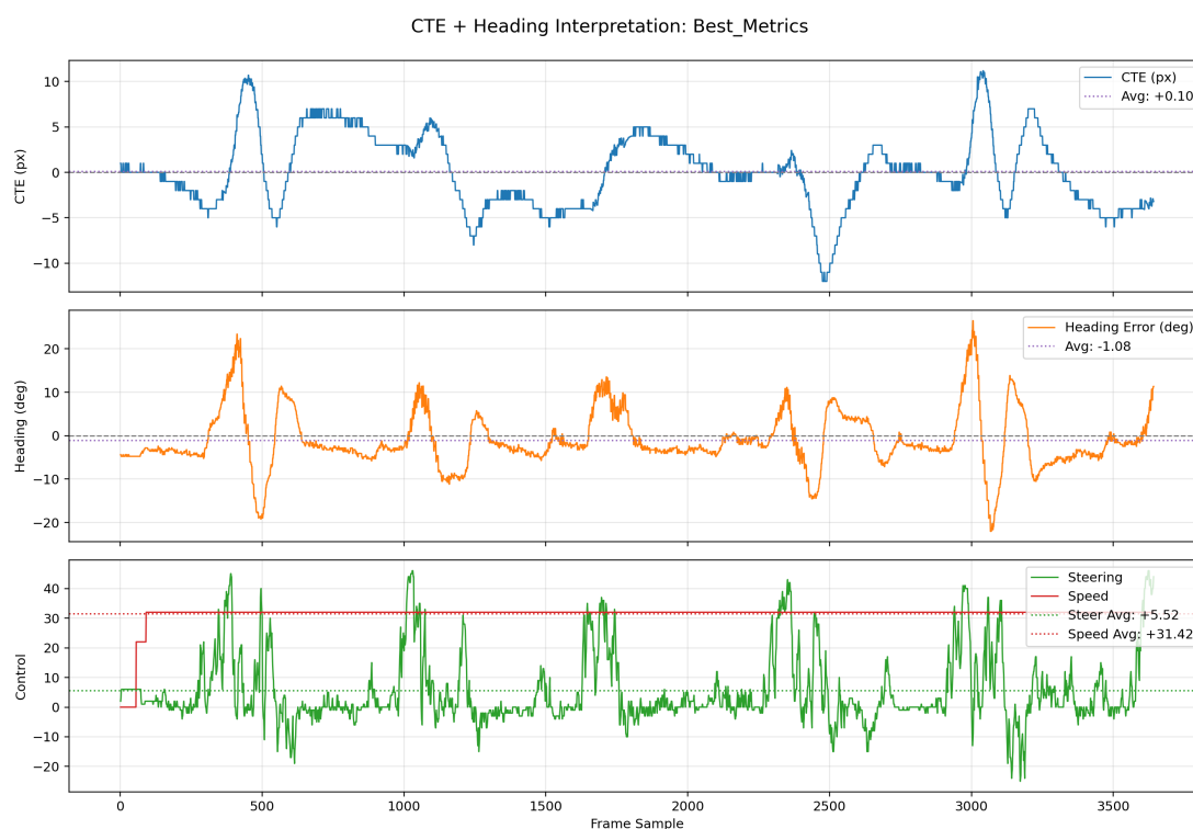
Figure 4.6: Physical deployment of the Egocentric Dynamic Crop Model resulted in successful navigation through the entire track, with stable CTE and Heading Error profiles.
