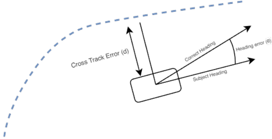
Figure 3.6: Visual representation of Cross-Track Error ( d ) and Heading Error ( \theta ).
