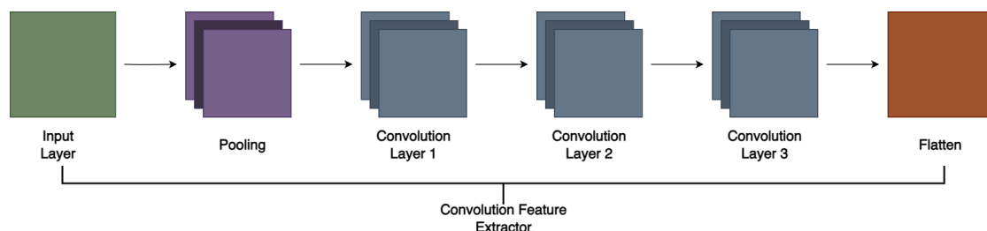
Figure 3.3: Feature Extraction Block: Input, Convolutional Layers, and Flattening
