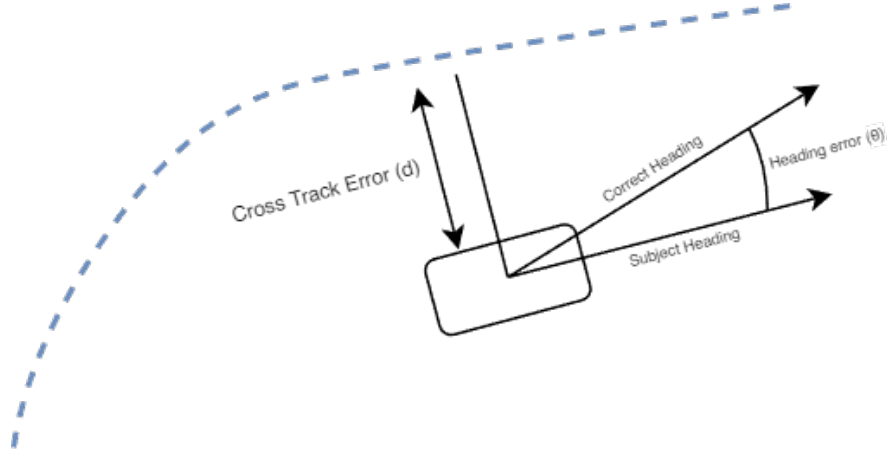
Figure 3.7: Visual representation of Cross-Track Error ( d ) and Heading Error ( \theta ).
