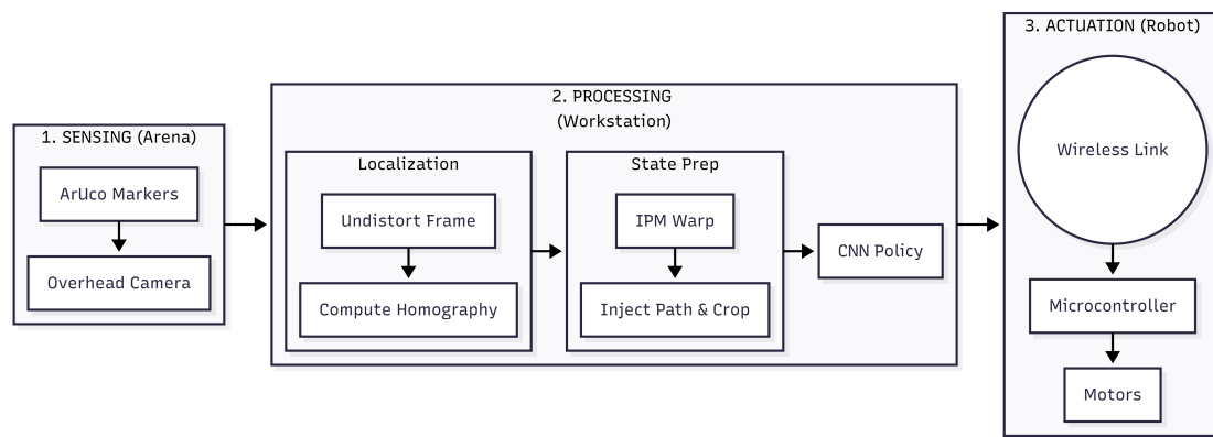
Figure 3.2: System Architecture.
