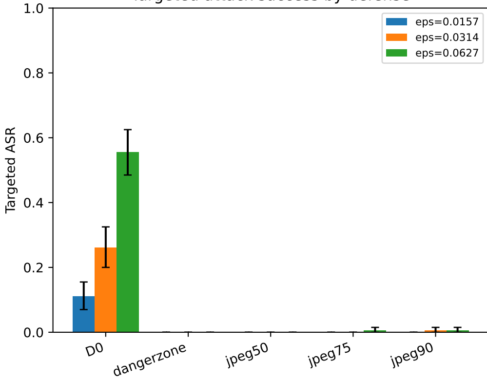
Targeted attack success by defense
