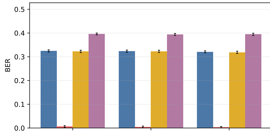
N288, M144: Decoded BER
