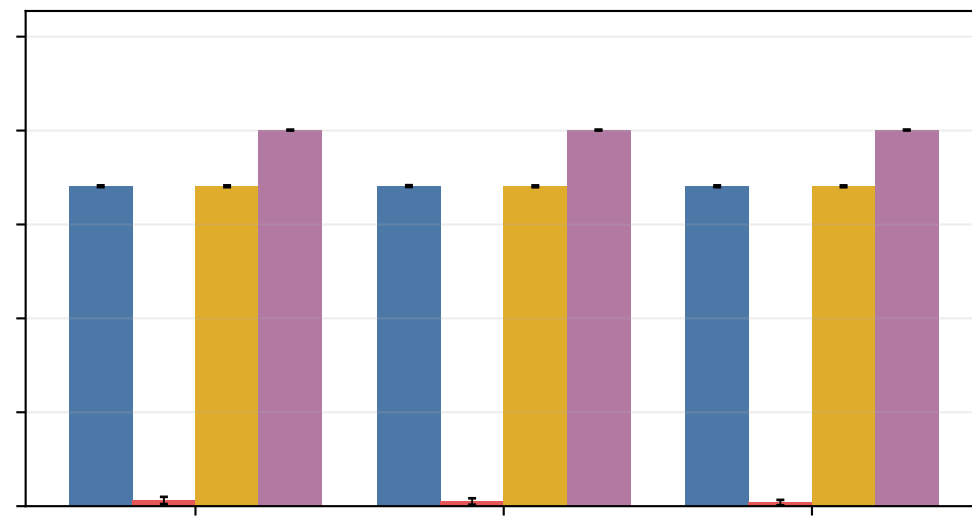
N288, M144: Late instantaneous BER
