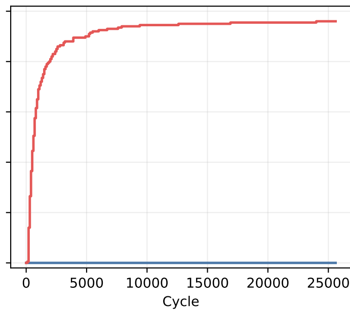
N288, Random
