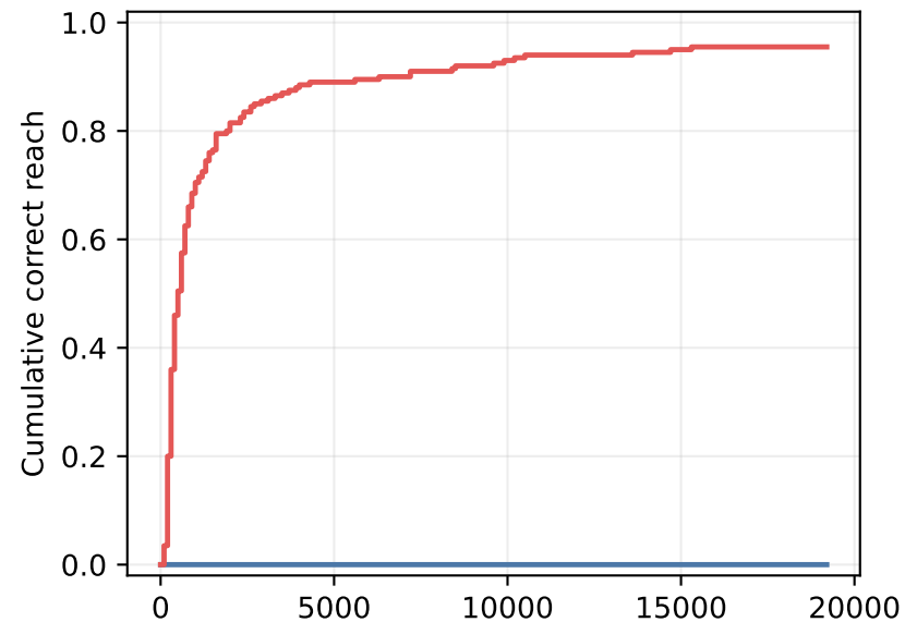
N192, All-zero
