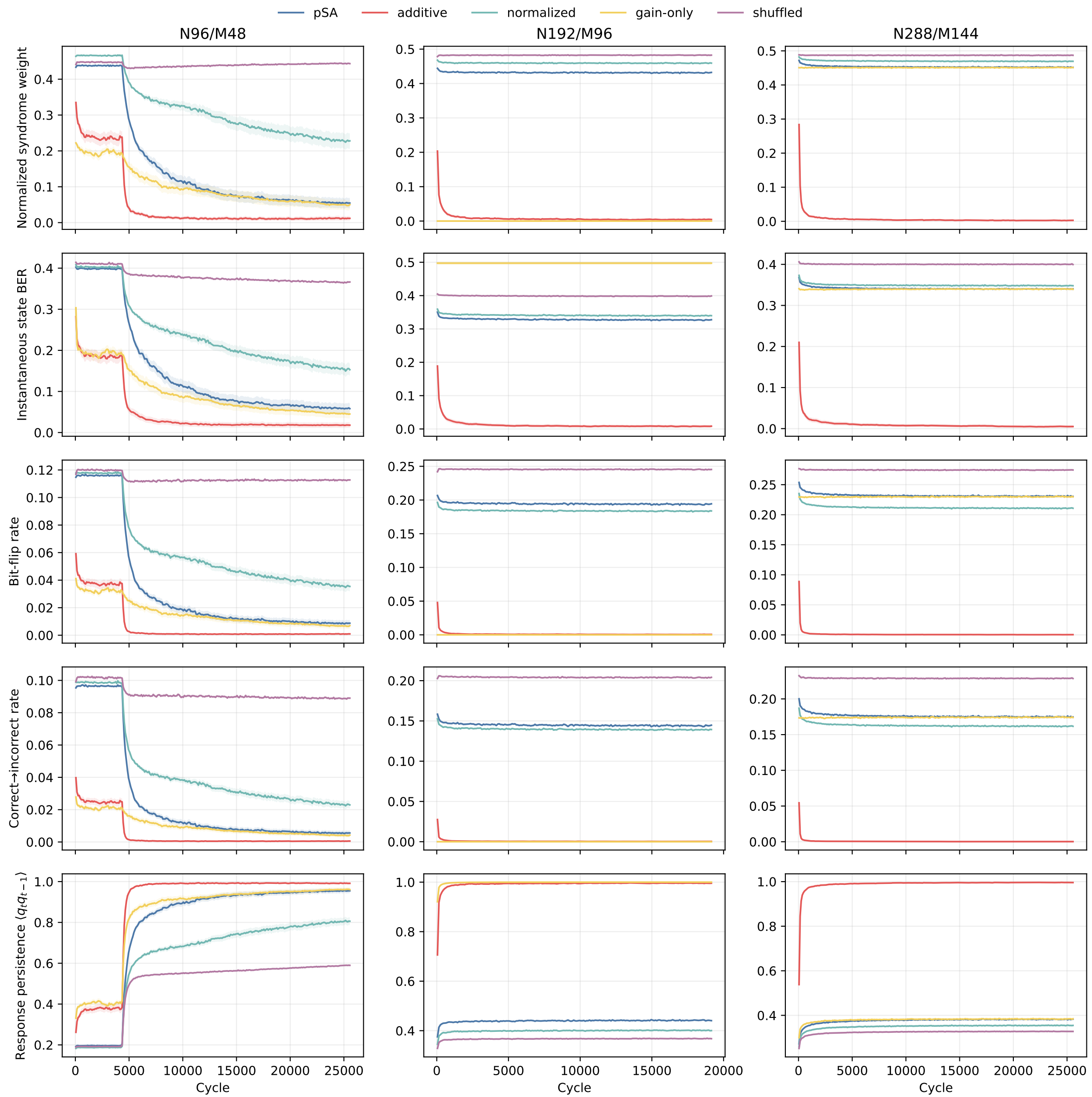
LDPC dynamics at E_b/N_0 = 2.5 dB
