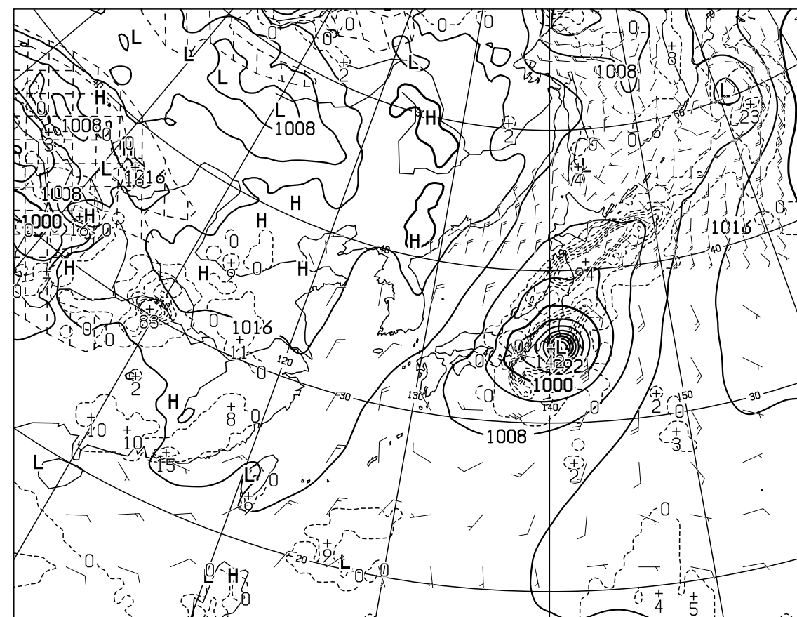
T=24 VALID 211200UTC SURFACE PRESS(hPa),PRECIP(MM) (12-24) WIND ARROW AT SURFACE
