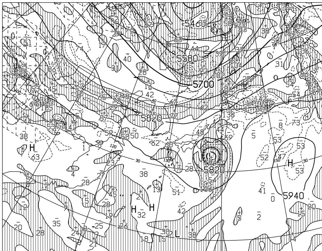
T=12 VALID 210000UTC HEIGHT(M),VORT(10 -6 /SEC) AT 500hPa
