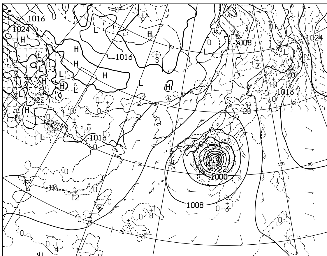
T=12 VALID 210000UTC SURFACE PRESS(hPa),PRECIP(MM) (00-12) WIND ARROW AT SURFACE
