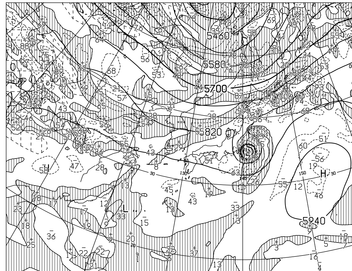
T=24 VALID 211200UTC HEIGHT(M),VORT(10 -6 /SEC) AT 500hPa
