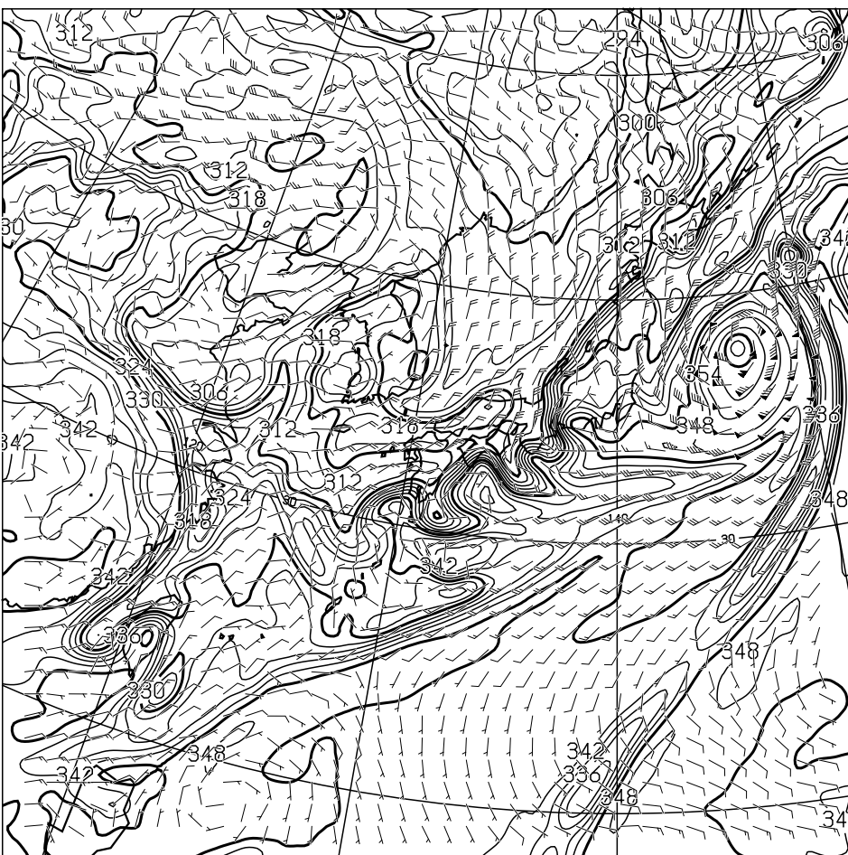
T=36 850hPa: E.P.TEMP(K),WIND(KNOTS) VALID 220000UTC
