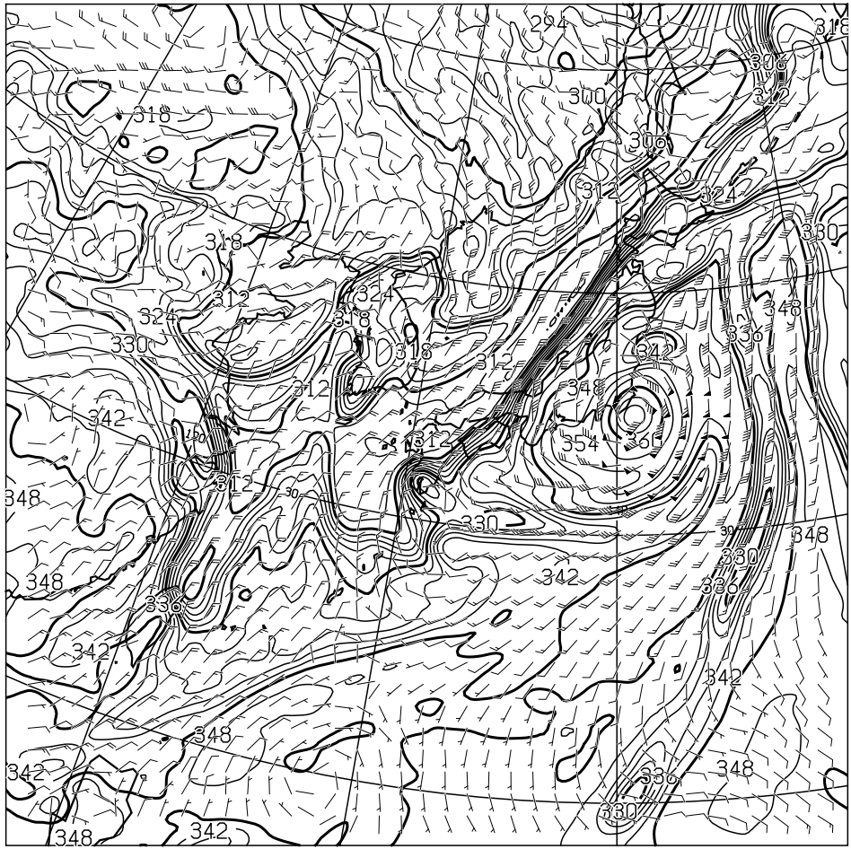
T=24 850hPa: E.P.TEMP(K),WIND(KNOTS) VALID 211200UTC
