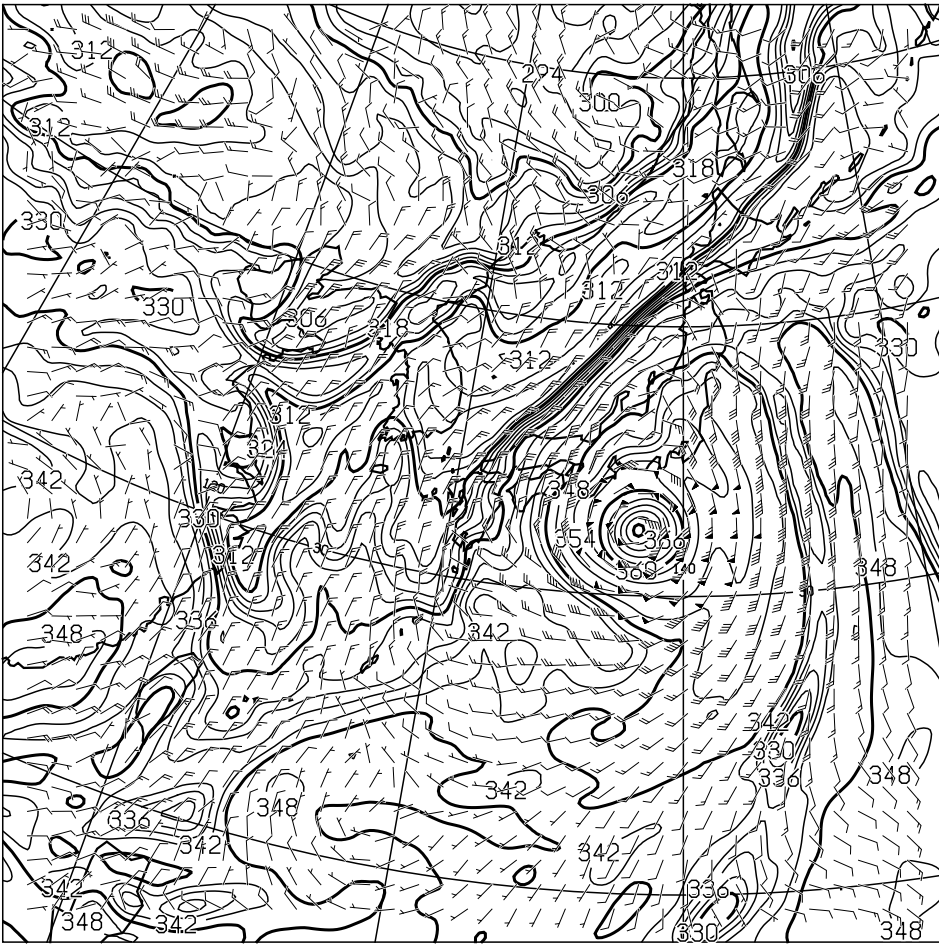
T=12 850hPa: E.P.TEMP(K),WIND(KNOTS) VALID 210000UTC
