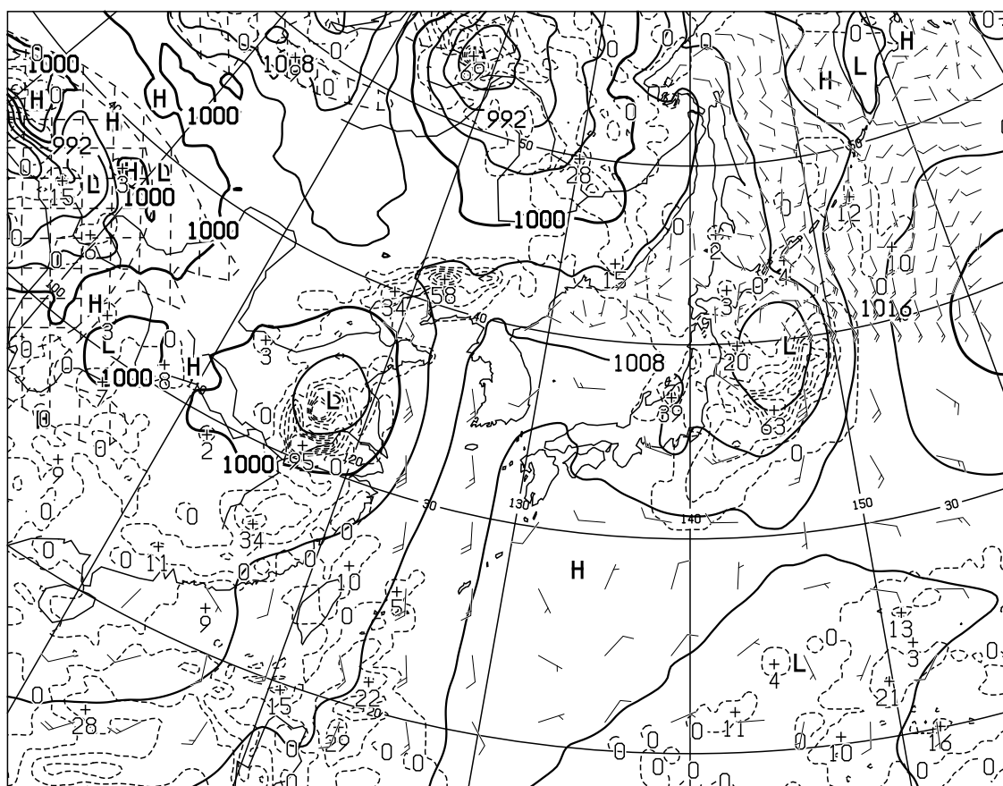
T=12 VALID 130000UTC SURFACE PRESS(hPa),PRECIP(MM) (00-12) WIND ARROW AT SURFACE
