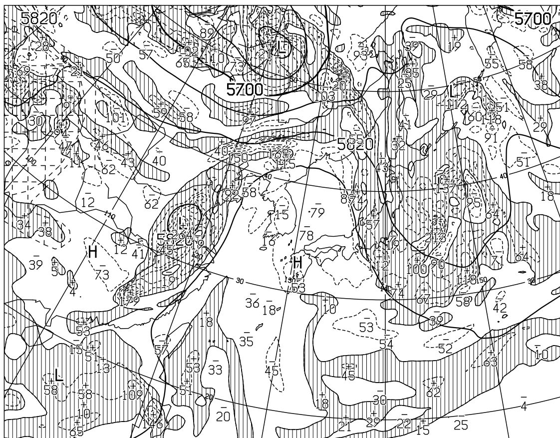
T=12 VALID 130000UTC HEIGHT(M),VORT(10**6/SEC) AT 500hPa
