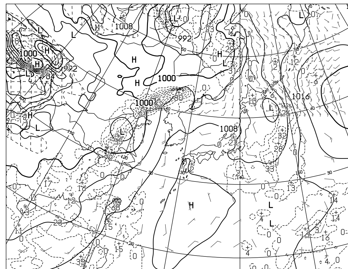
T=24 VALID 131200UTC SURFACE PRESS(hPa),PRECIP(MM) (12-24) WIND ARROW AT SURFACE
