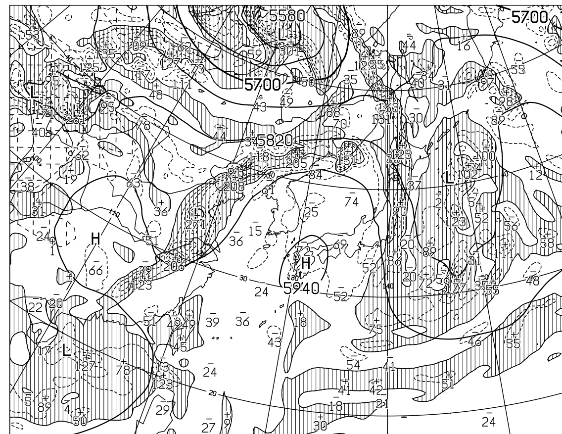
T=24 VALID 131200UTC HEIGHT(M),VORT(10**6/SEC) AT 500hPa
