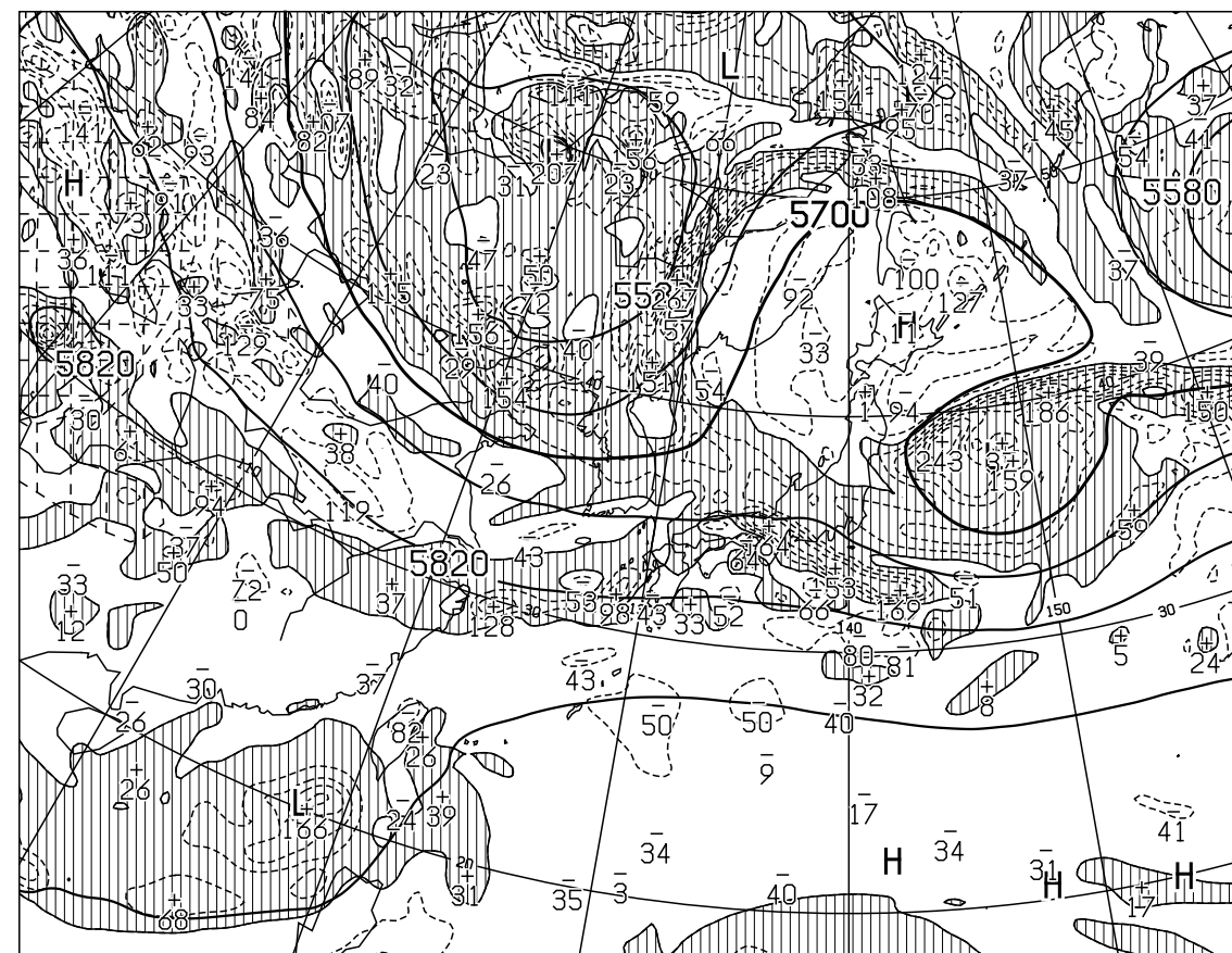
T=24 VALID 041200UTC HEIGHT(M),VORT(10**6/SEC) AT 500hPa
