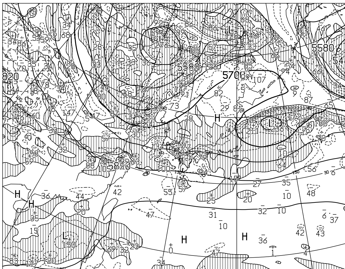
T=12 VALID 040000UTC HEIGHT(M),VORT(10**6/SEC) AT 500hPa
