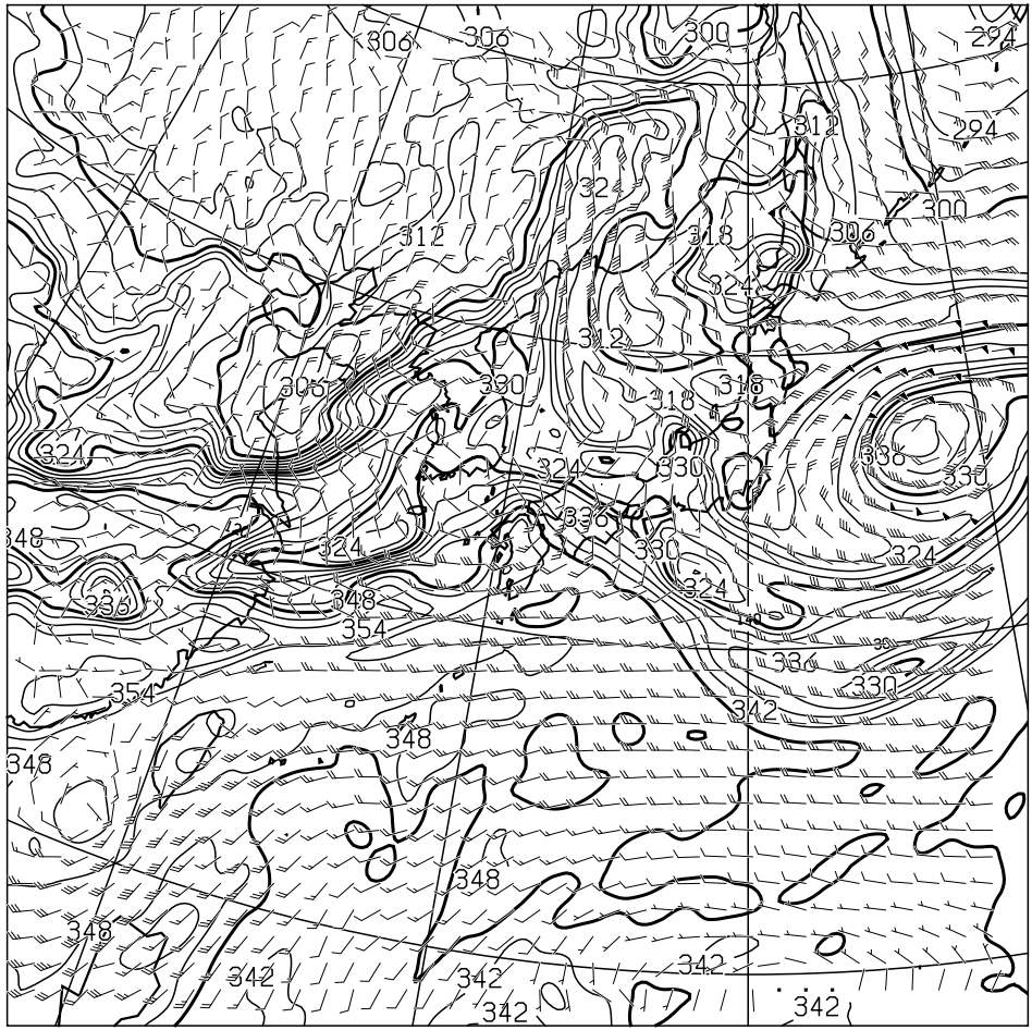
T=24 850hPa: E.P.TEMP(K),WIND(KNOTS) VALID 041200UTC
