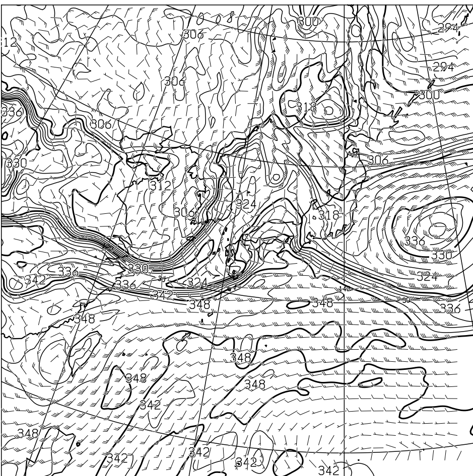
T=36 850hPa: E.P.TEMP(K),WIND(KNOTS) VALID 050000UTC
