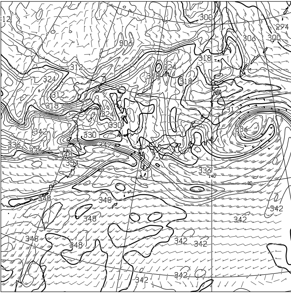
T=12 850hPa: E.P.TEMP(K),WIND(KNOTS) VALID 040000UTC
