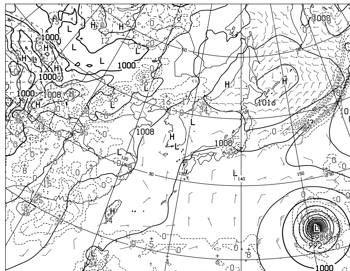
T=24 VALID 021200UTC SURFACE PRESS(hPa),PRECIP(MM) (12-24) WIND ARROW AT SURFACE
