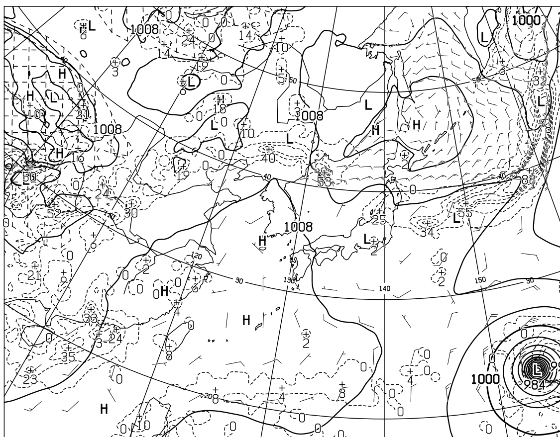
T=12 VALID 020000UTC SURFACE PRESS(hPa),PRECIP(MM) (00-12) WIND ARROW AT SURFACE
