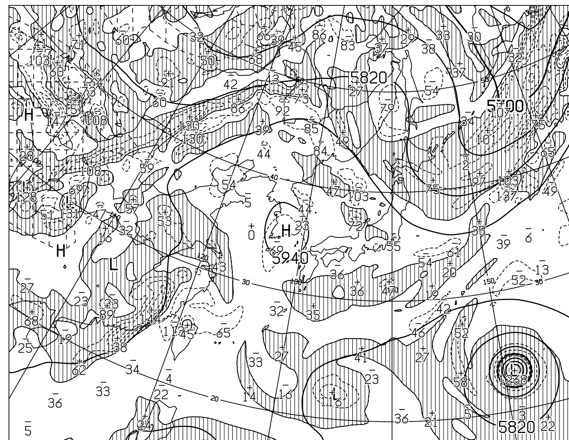
T=24 VALID 021200UTC HEIGHT(M),VORT(10×-6/SEC) AT 500hPa
