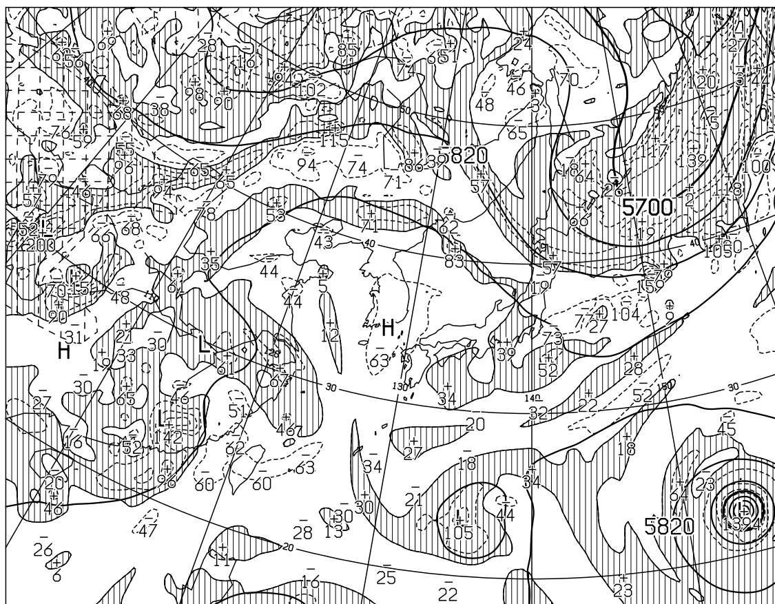
T=12 VALID 020000UTC HEIGHT(M),VORT(10×-6/SEC) AT 500hPa
