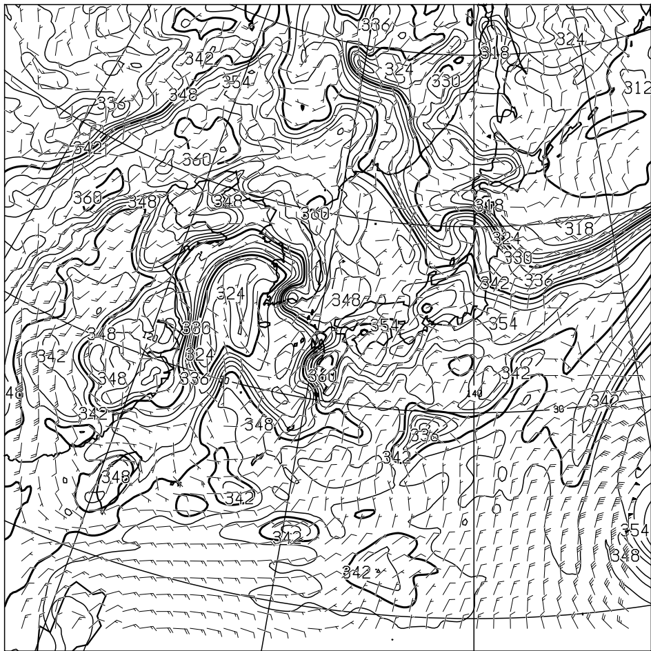
T=24 850hPa: E.P.TEMP(K),WIND(KNOTS) VALID 021200UTC
