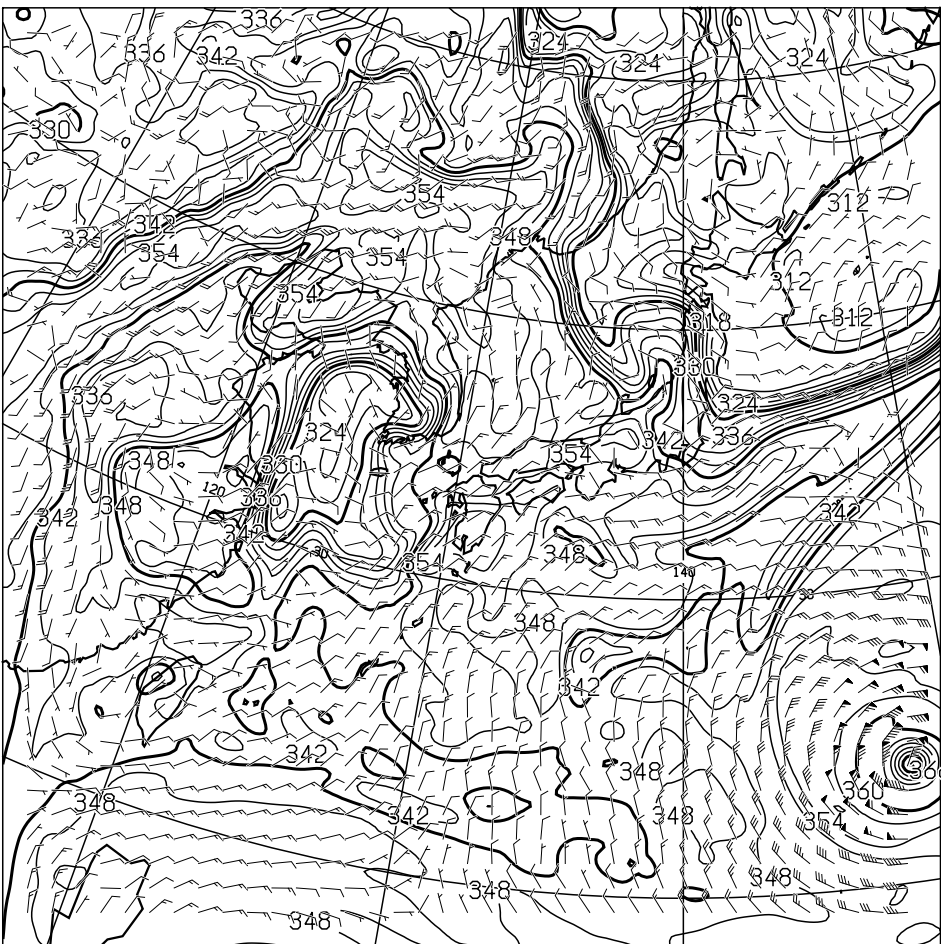
T=36 850hPa: E.P.TEMP(K),WIND(KNOTS) VALID 030000UTC
