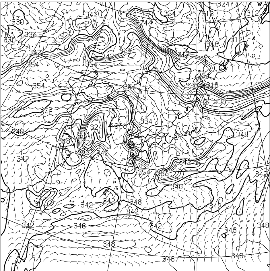
T=12 850hPa: E.P.TEMP(K),WIND(KNOTS) VALID 020000UTC
