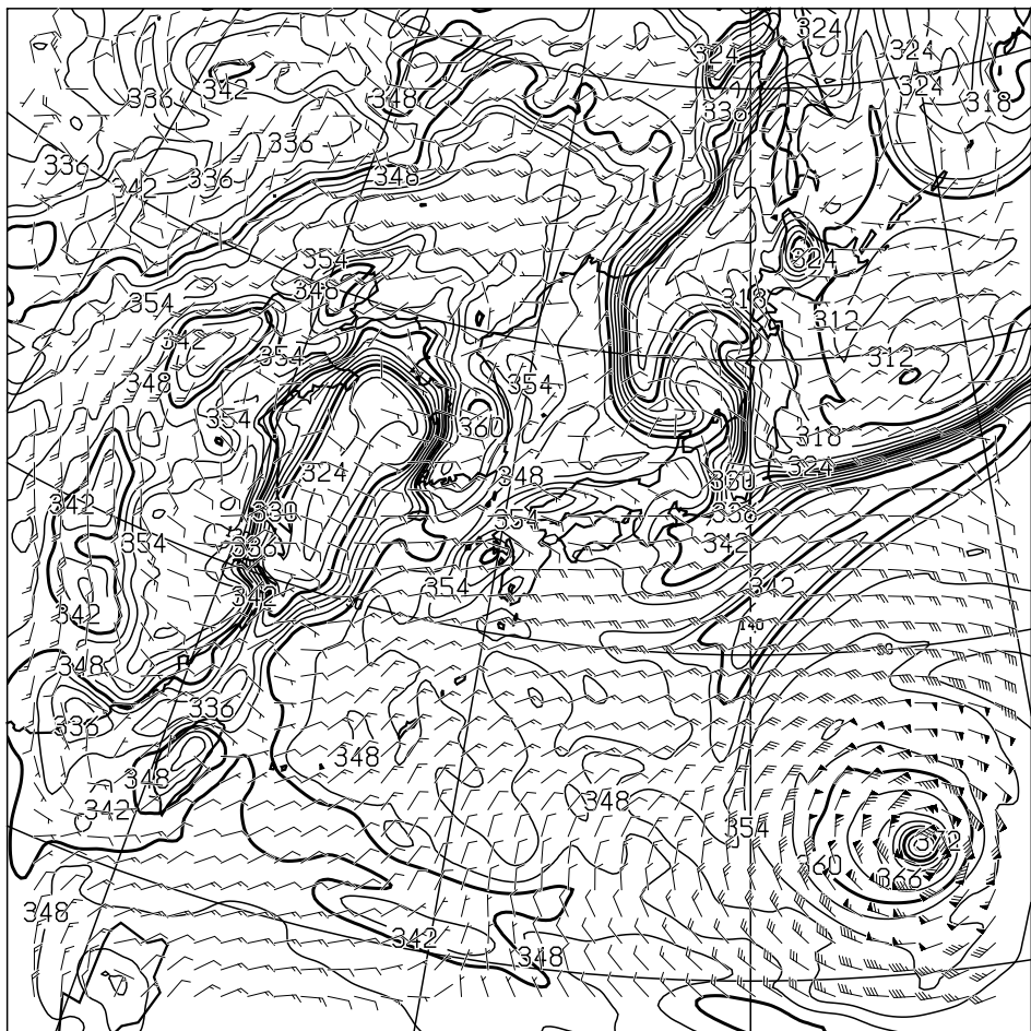
T=48 850hPa: E.P.TEMP(K),WIND(KNOTS) VALID 031200UTC
